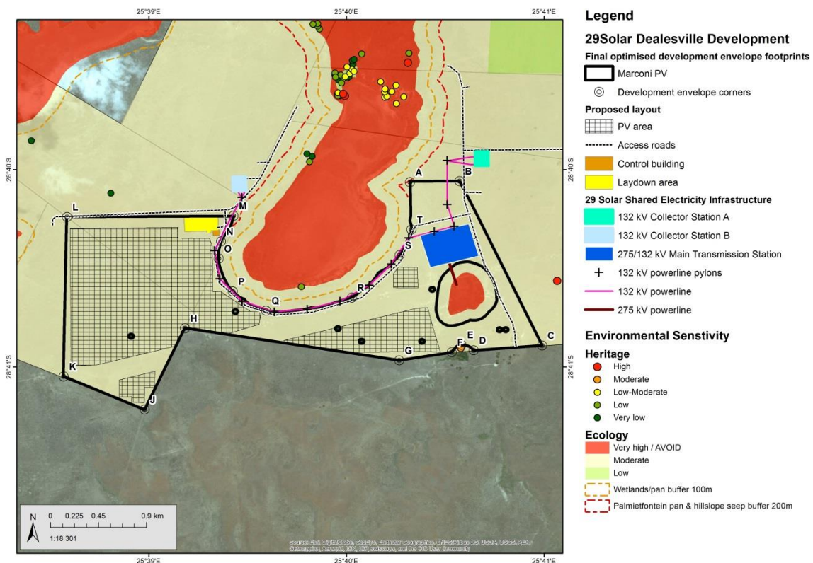
Environmental sensitivity map indicating the Marconi PV development envelope with proposed technical layout, which avoids all environmental sensitivities.
