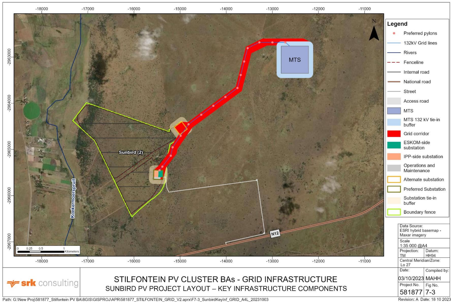
Figure 7-3: Sunbird Grid infrastructure layout – key infrastructure components
