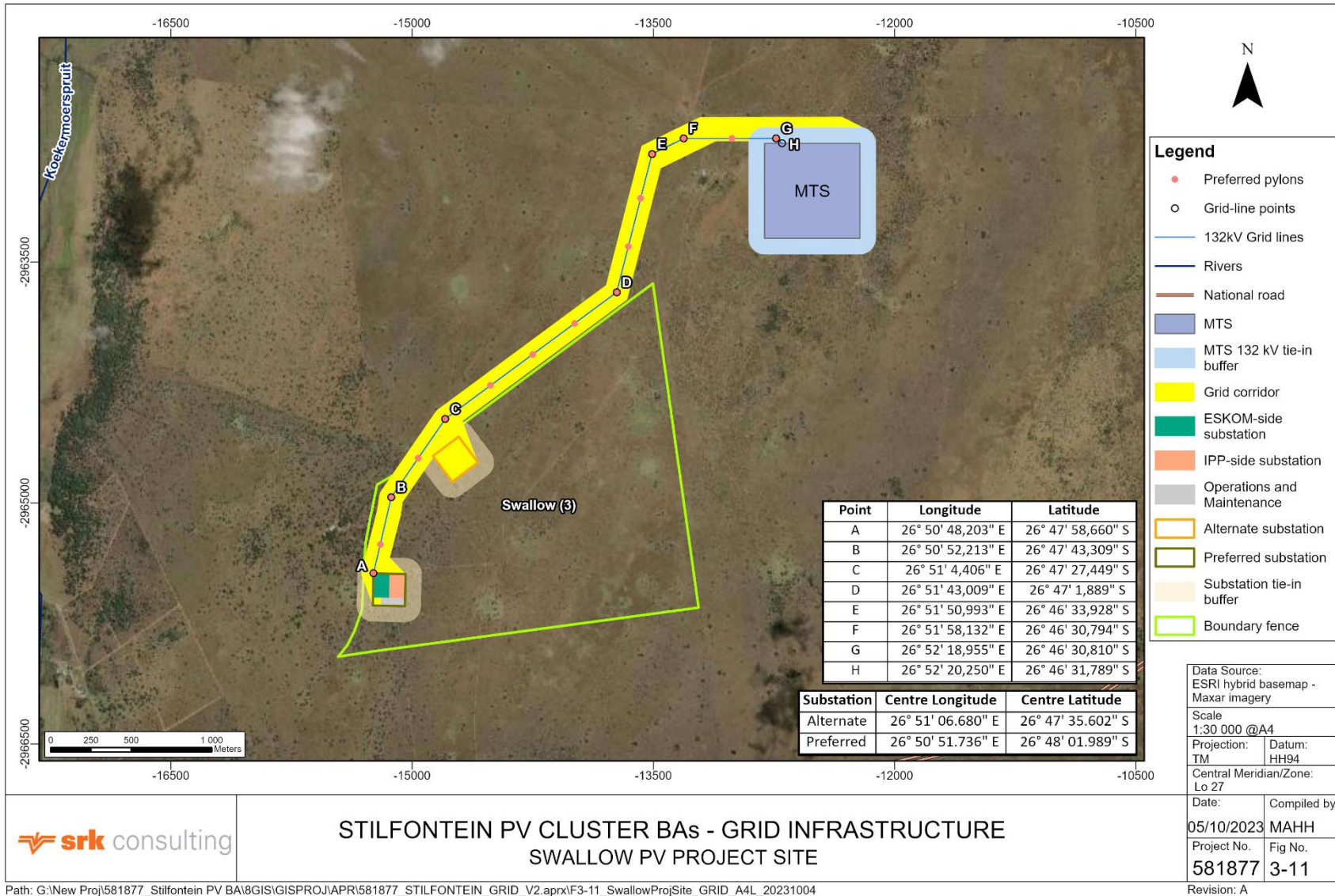
Figure 3-11: Layout of Swallow project
