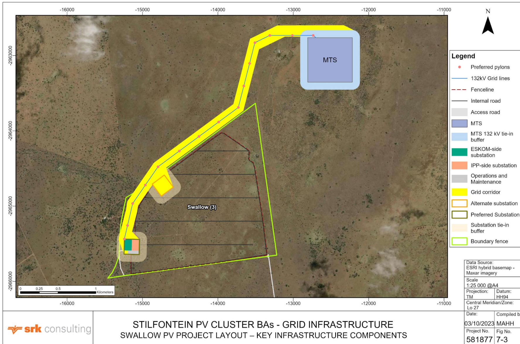
Figure 7-3: Swallow Grid infrastructure layout – key infrastructure components
