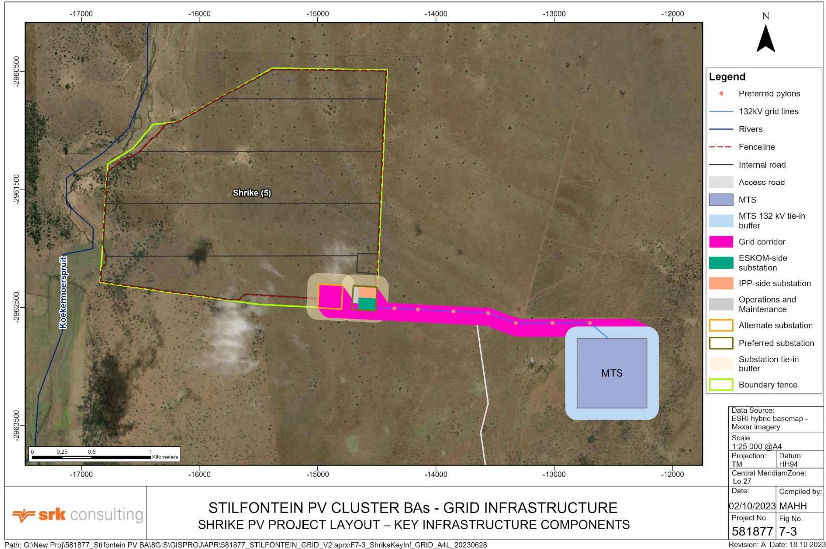
Figure 7-3: Shrike Grid infrastructure layout – key infrastructure components
