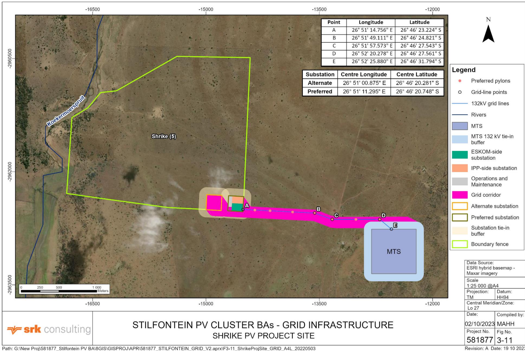
Figure 3-11: Layout of Shrike project
