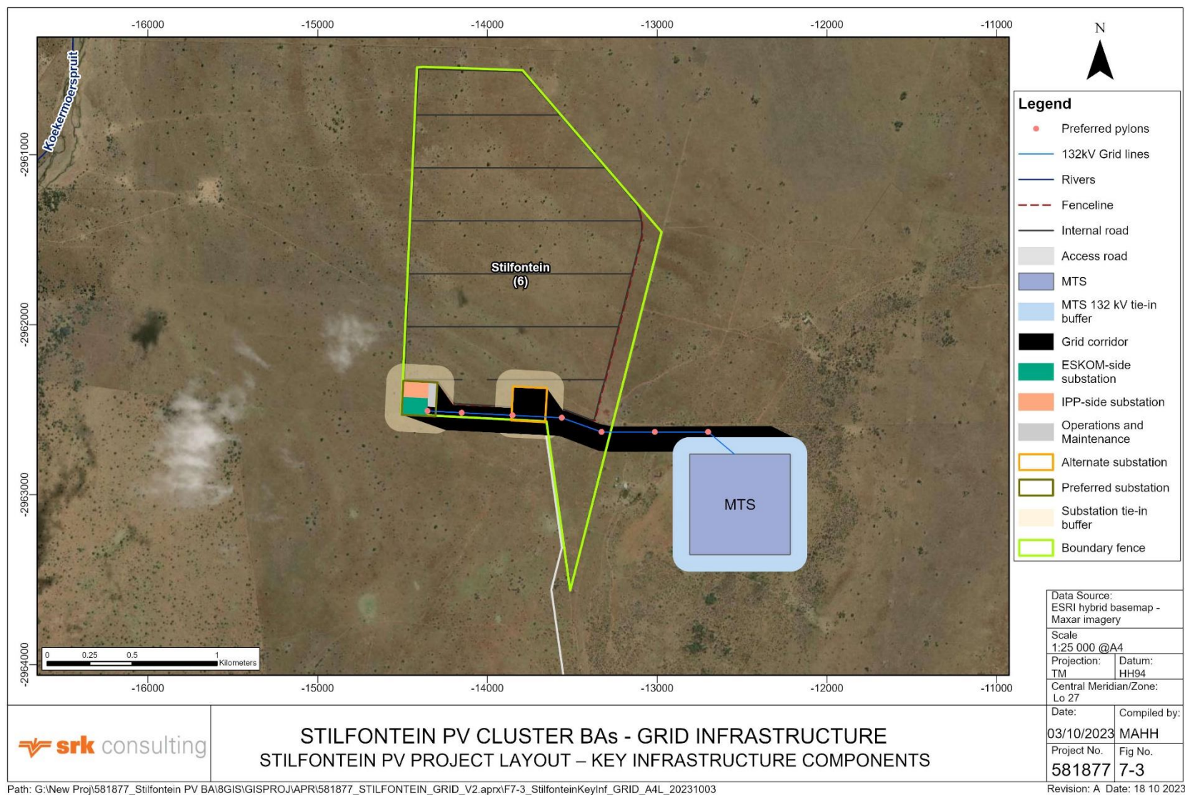
Figure 7-3: Stilfontein Grid infrastructure layout – key infrastructure components
