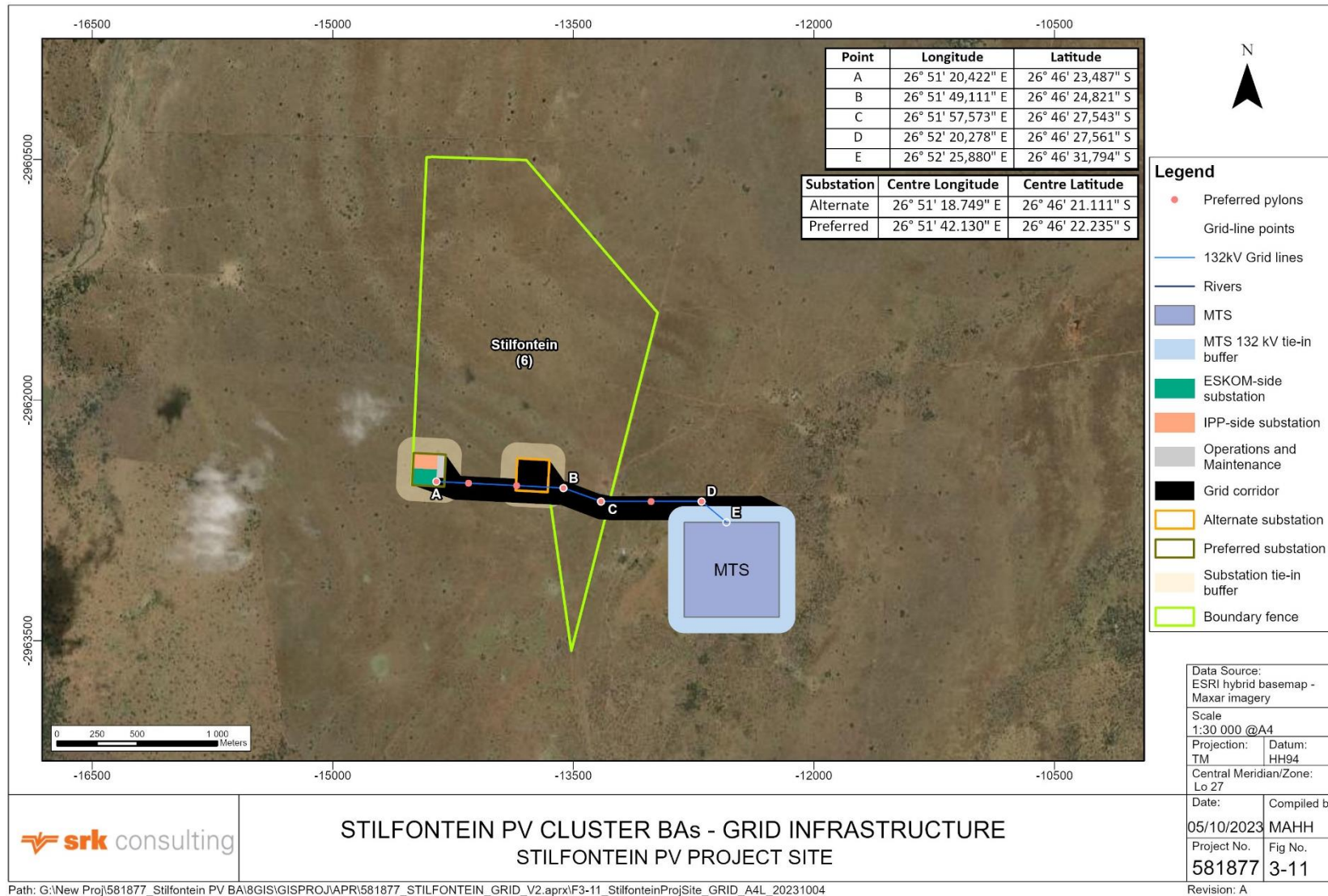
Figure 3-11: Layout of Stilfontein Project
