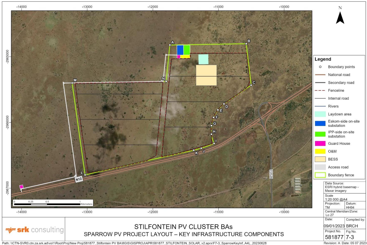
Figure 7-3: Sparrow PV project layout - key infrastructure components 48
