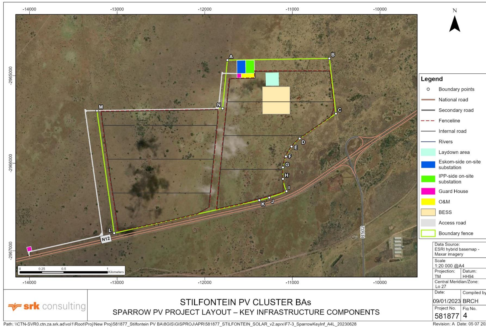
Figure 4: Sparrow PV project layout – key infrastructure components 2
