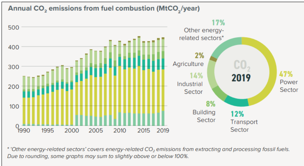
Figure 3-8: Annual CO 2 emissions from fuel combustion in South Africa (million tons / year)
