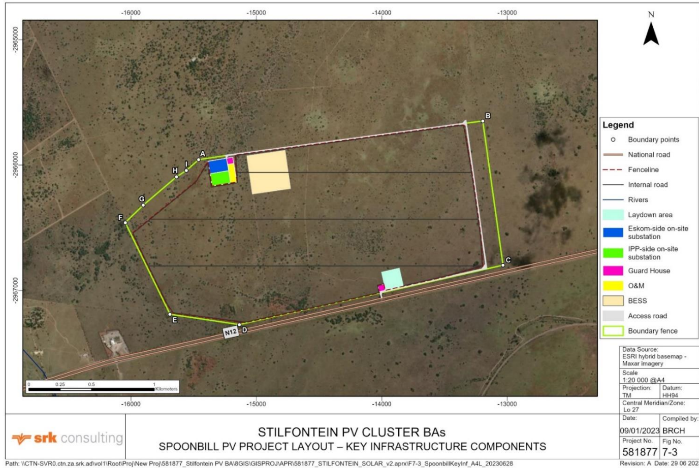
Figure 7-3: Spoonbill PV Project Layout – key infrastructure components 49
