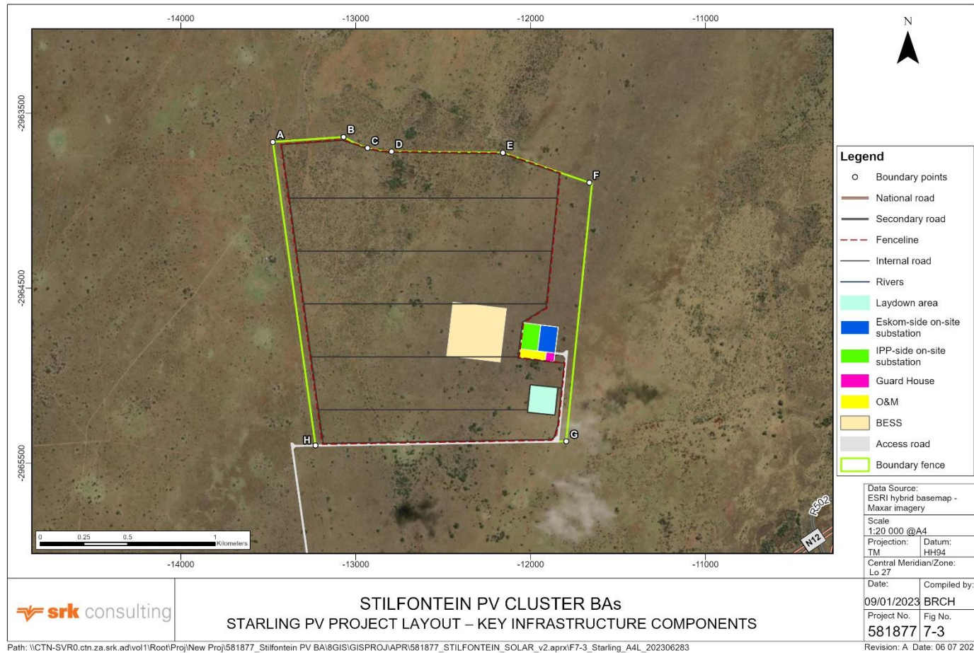
Figure 7-3: Starling PV project layout - key infrastructure components 47
