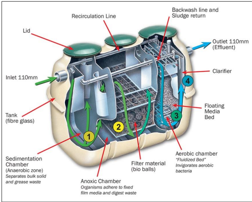
Figure 3-19: Schematic of a wastewater treatment unit
