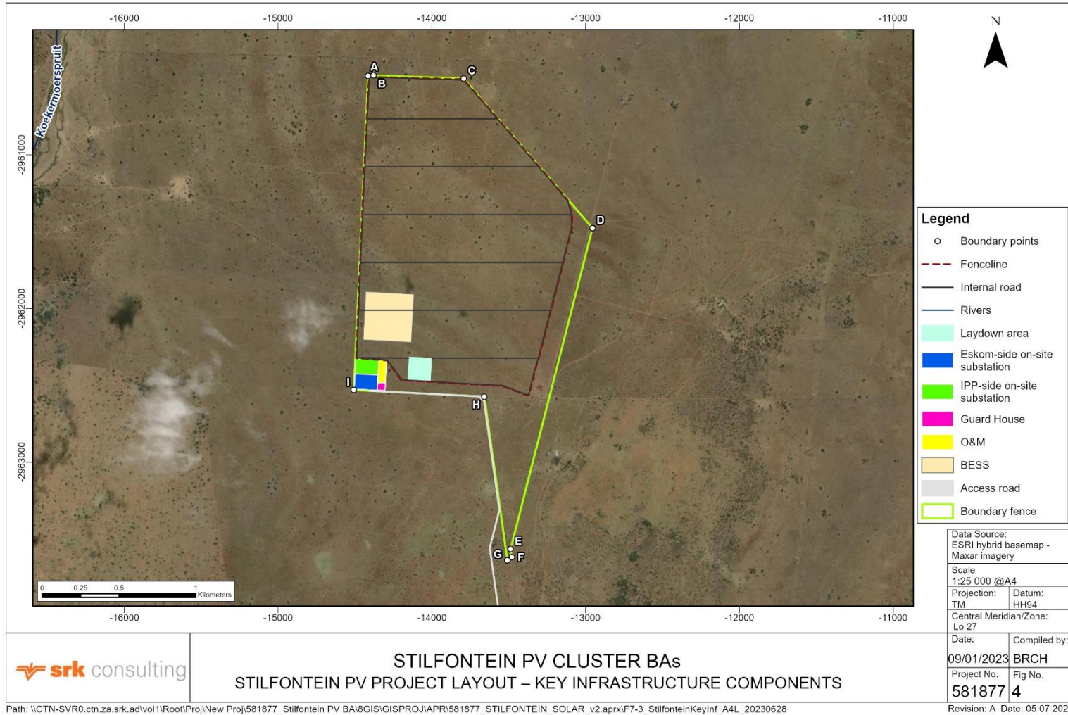
Figure 4: Stilfontein PV project layout – key infrastructure components 2
