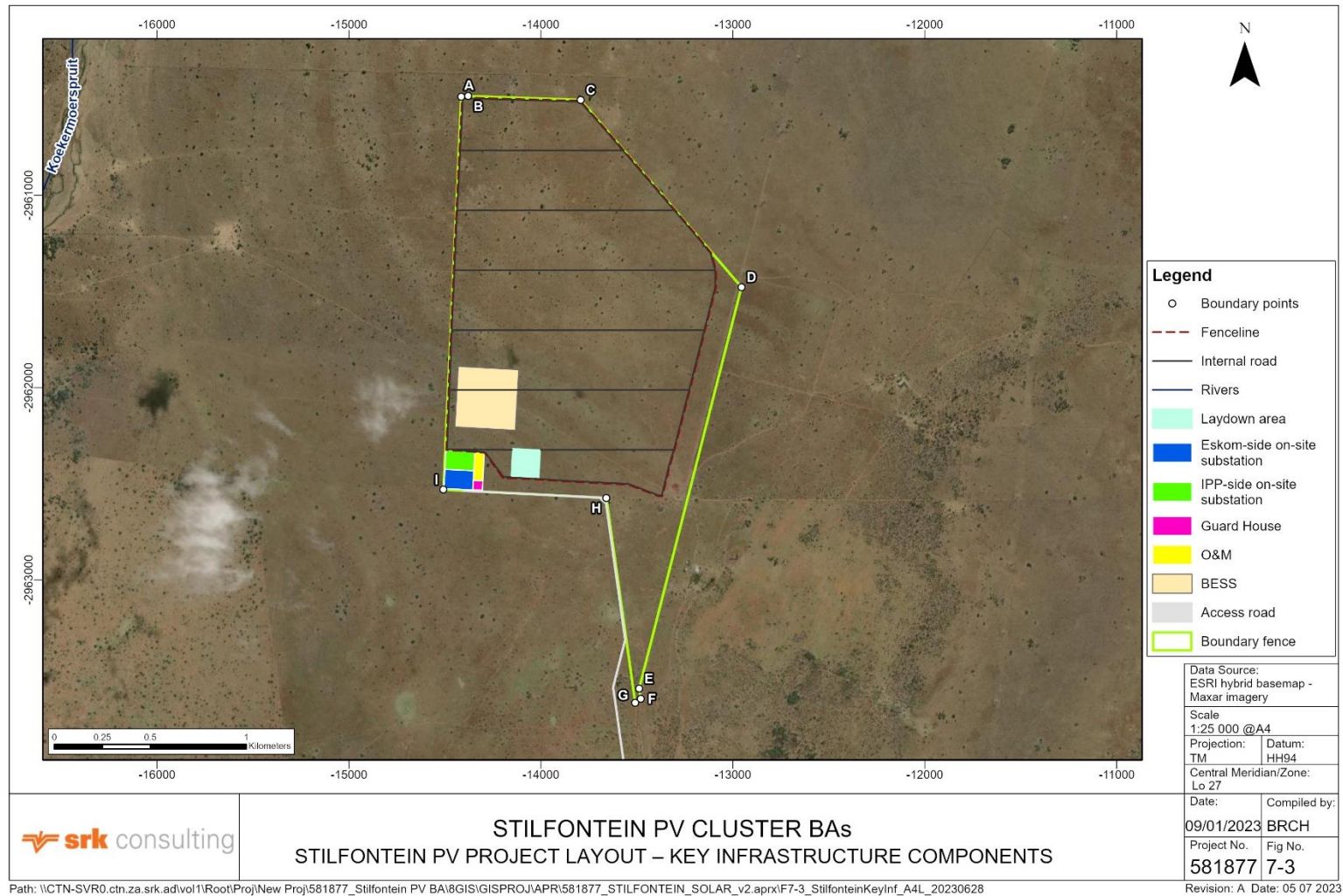
Figure 7-3: Stilfontein PV Project Layout – key infrastructure components 48
