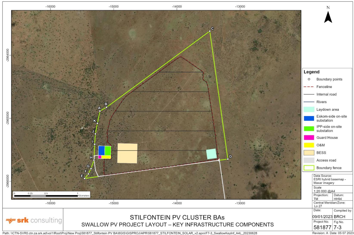
Figure 7-3: Swallow PV project layout - key infrastructure components 49
