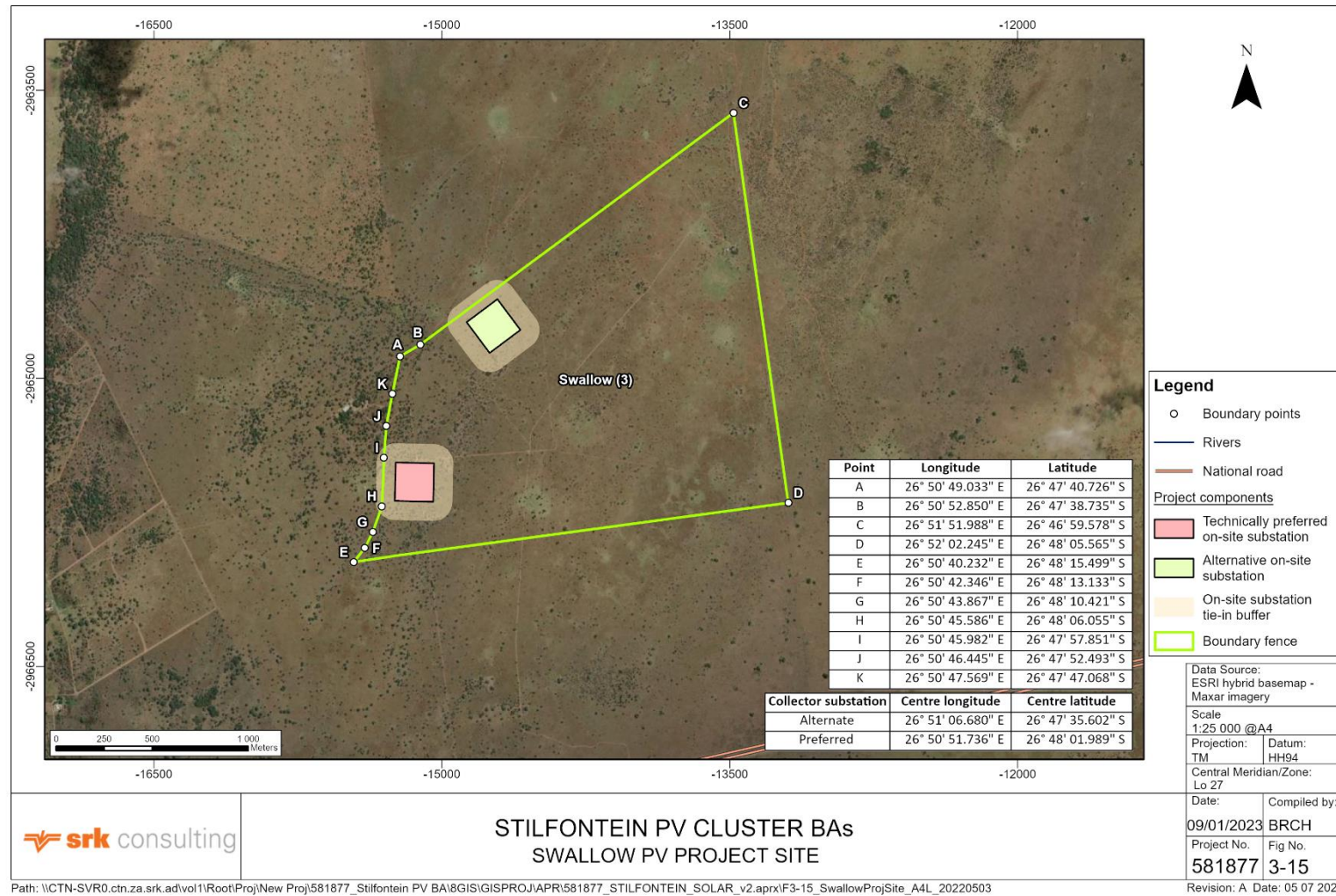
Figure 3-15: Swallow PV project site 20
