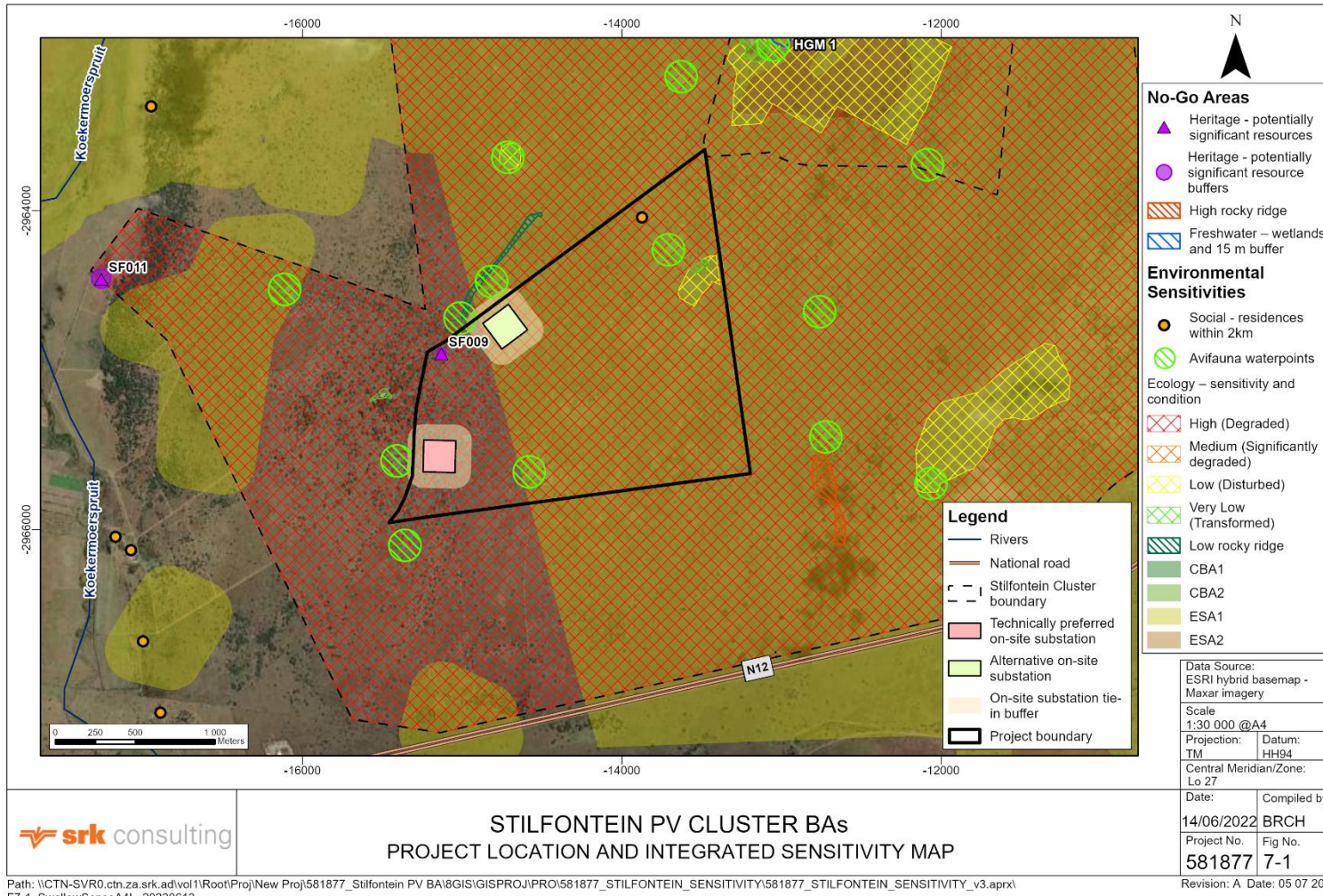
Figure 7-1: Integrated sensitivity map: Swallow
