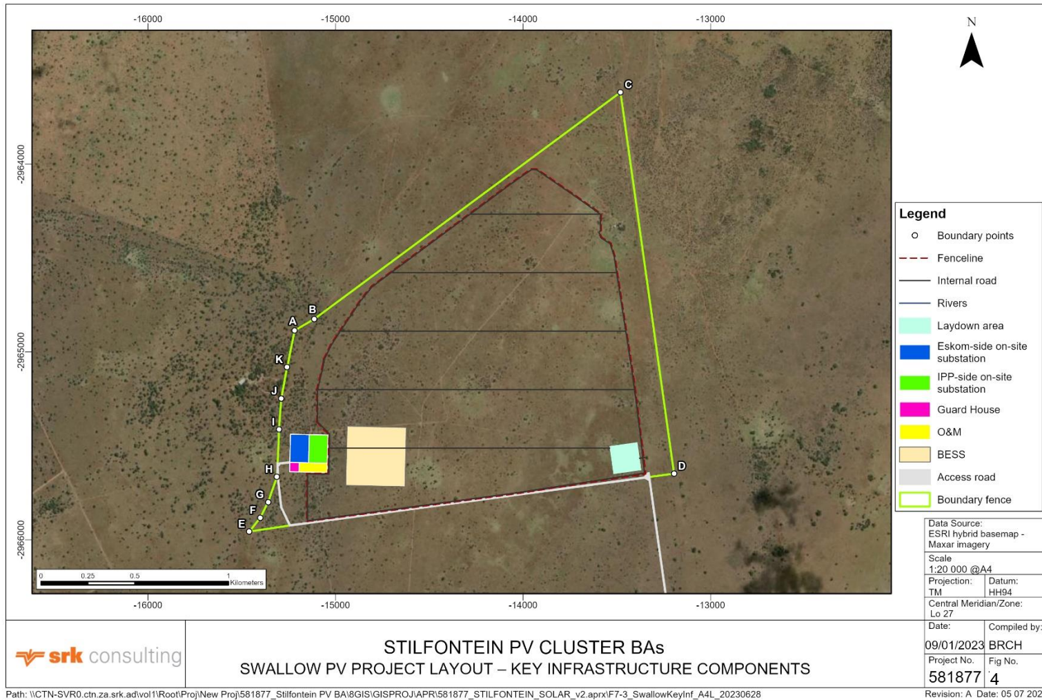
Figure 4: Swallow PV project layout – key infrastructure components 2
