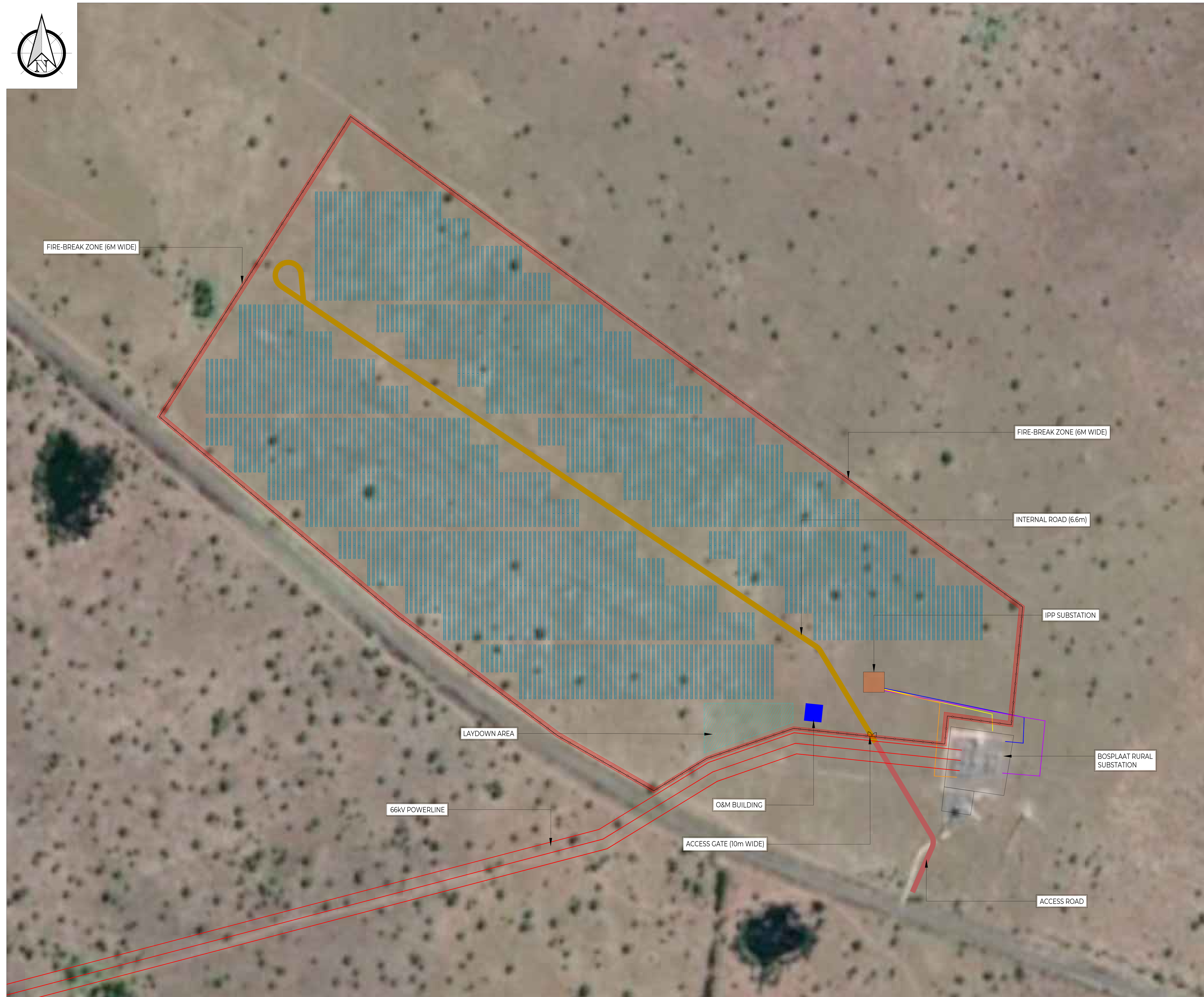
PLANT OVERVIEW SCALE 1:1500
