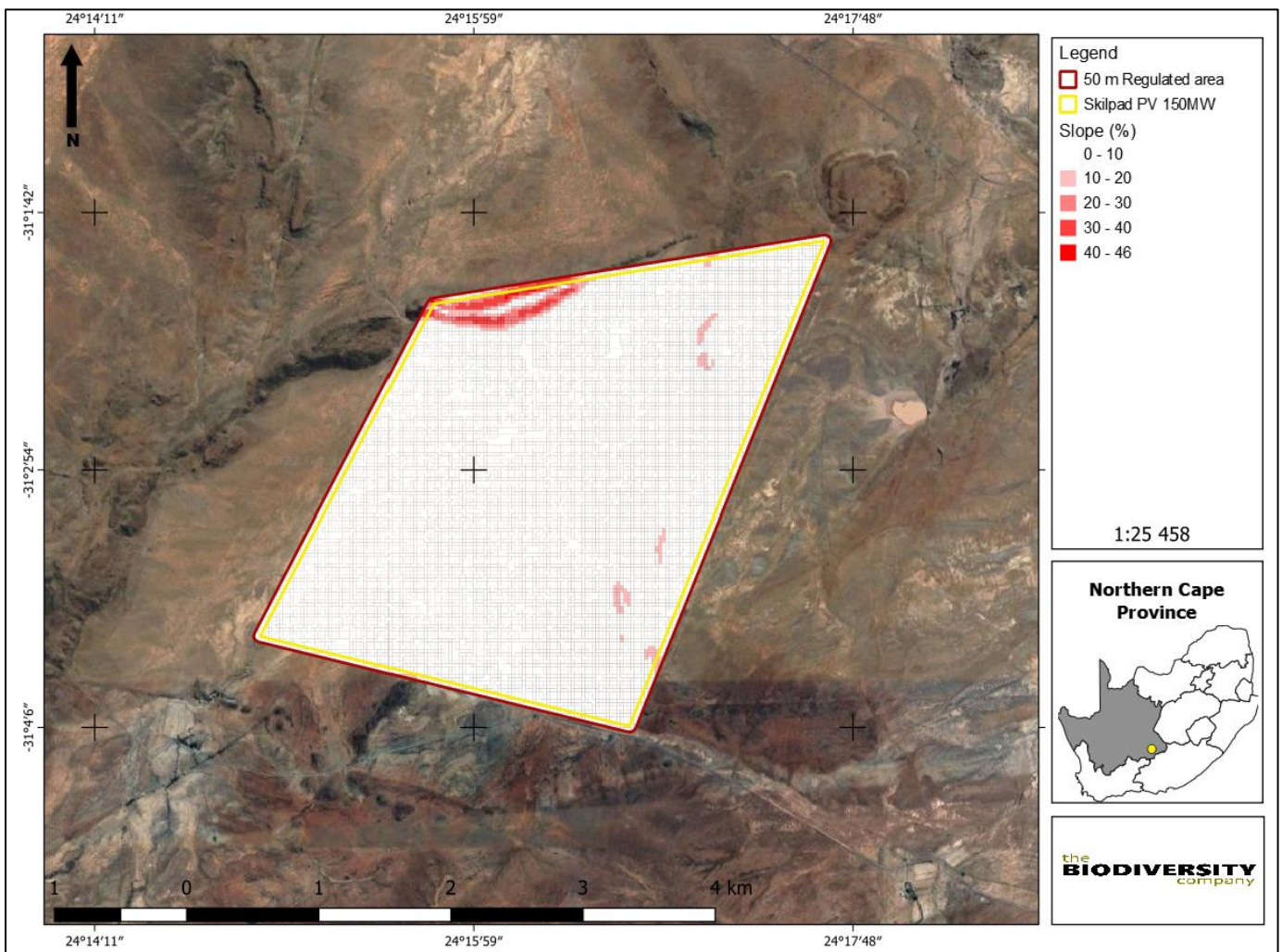
Figure 4-4: Slope percentage for the Skilpad SEF development area
