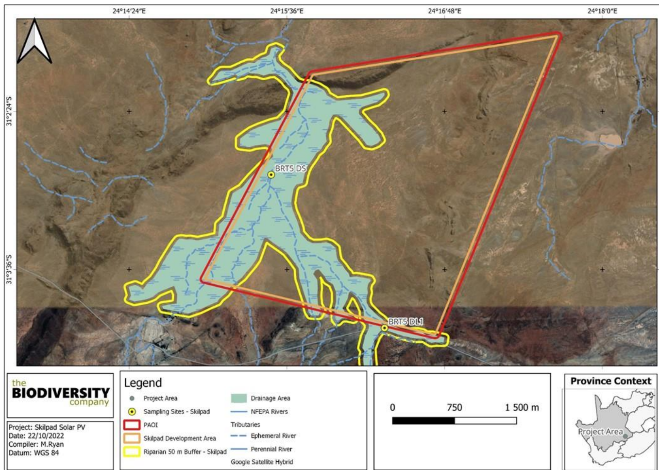
Figure 4-8: Riparian zones and associated 50 m buffers in the Skilpad SEF development area
