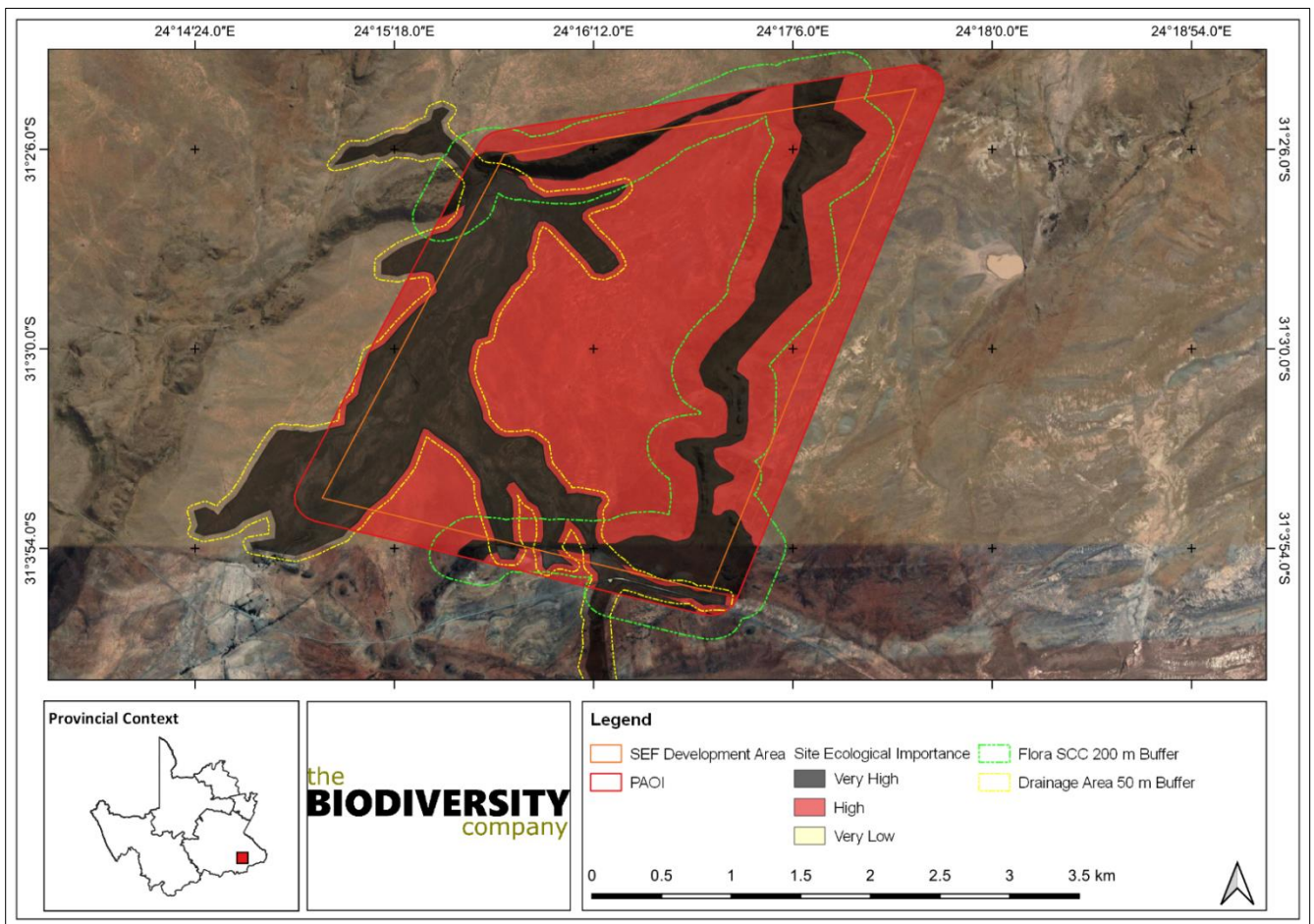
Figure 4-13: Site ecological importance of habitats in Skilpad SEF development area
