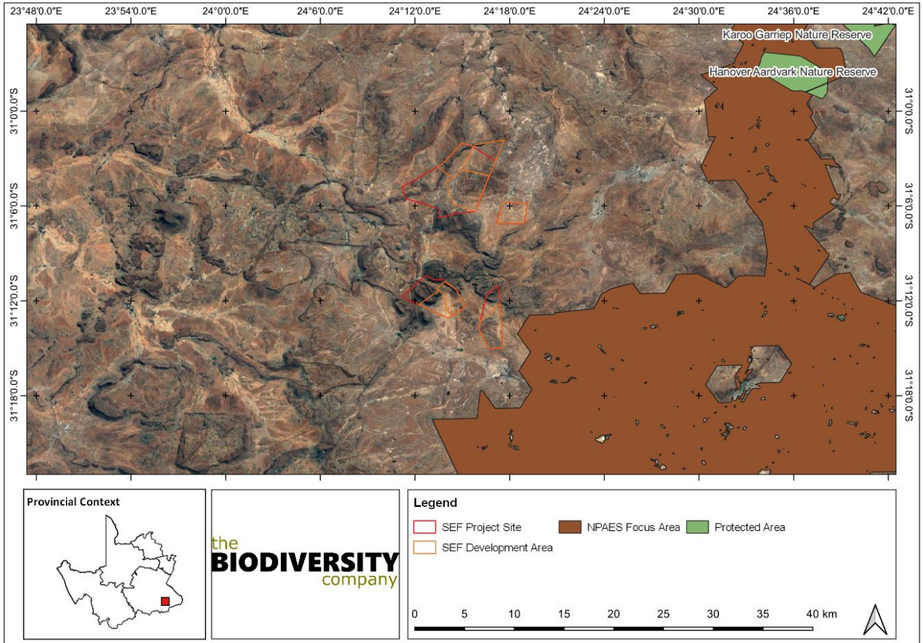
Figure 4-11: Skilpad SEF in relation to Protected Areas and NPAES Focus Areas
