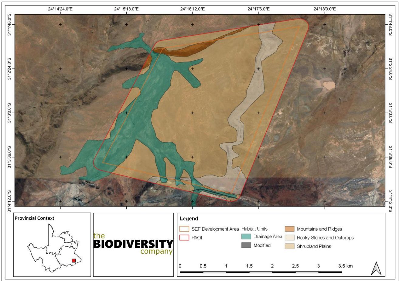
Figure 4-12: Habitat units in Skilpad SEF development area
