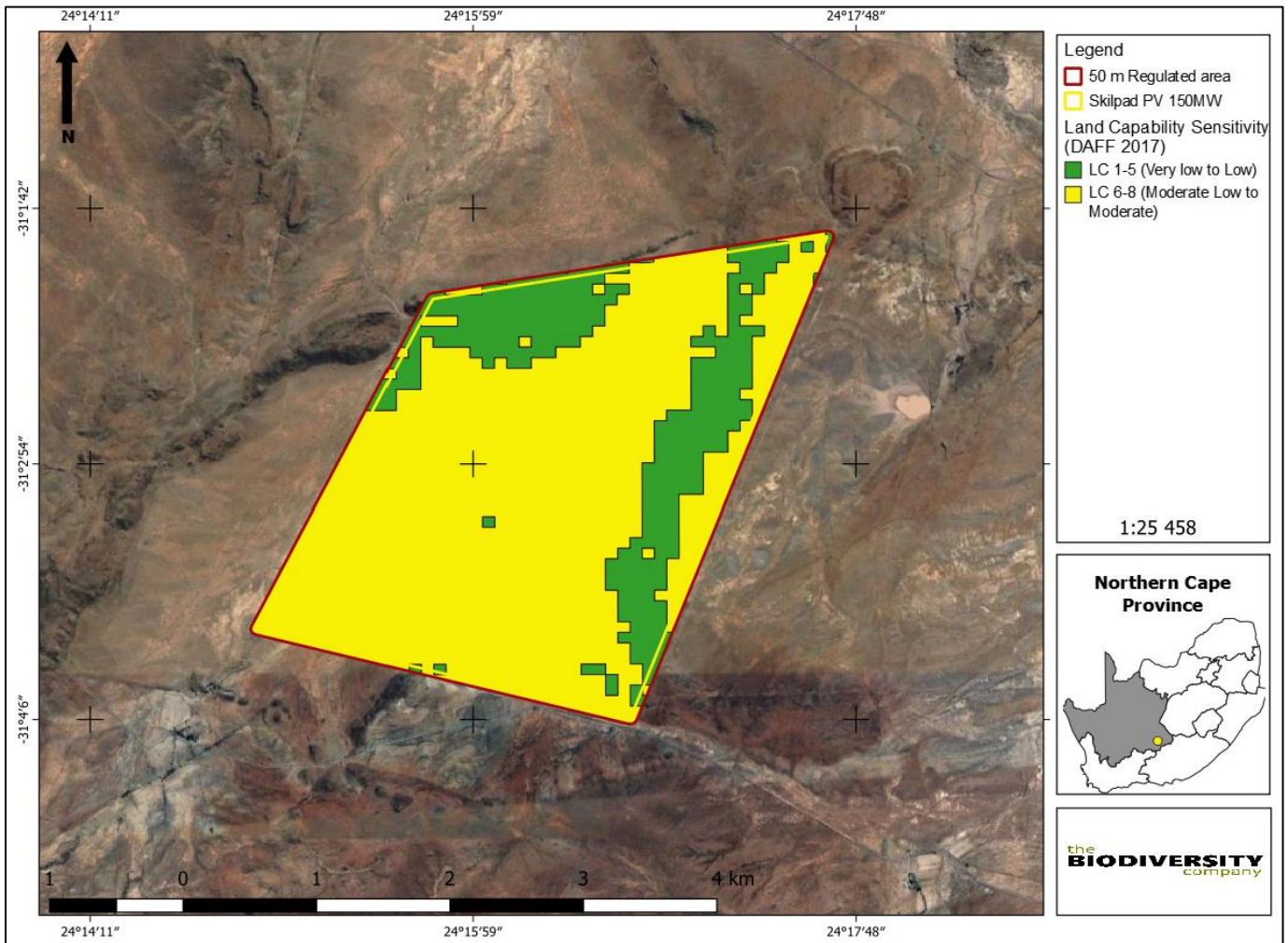
Figure 4-6: Land capability sensitivity of the Skilpad SEF development area
