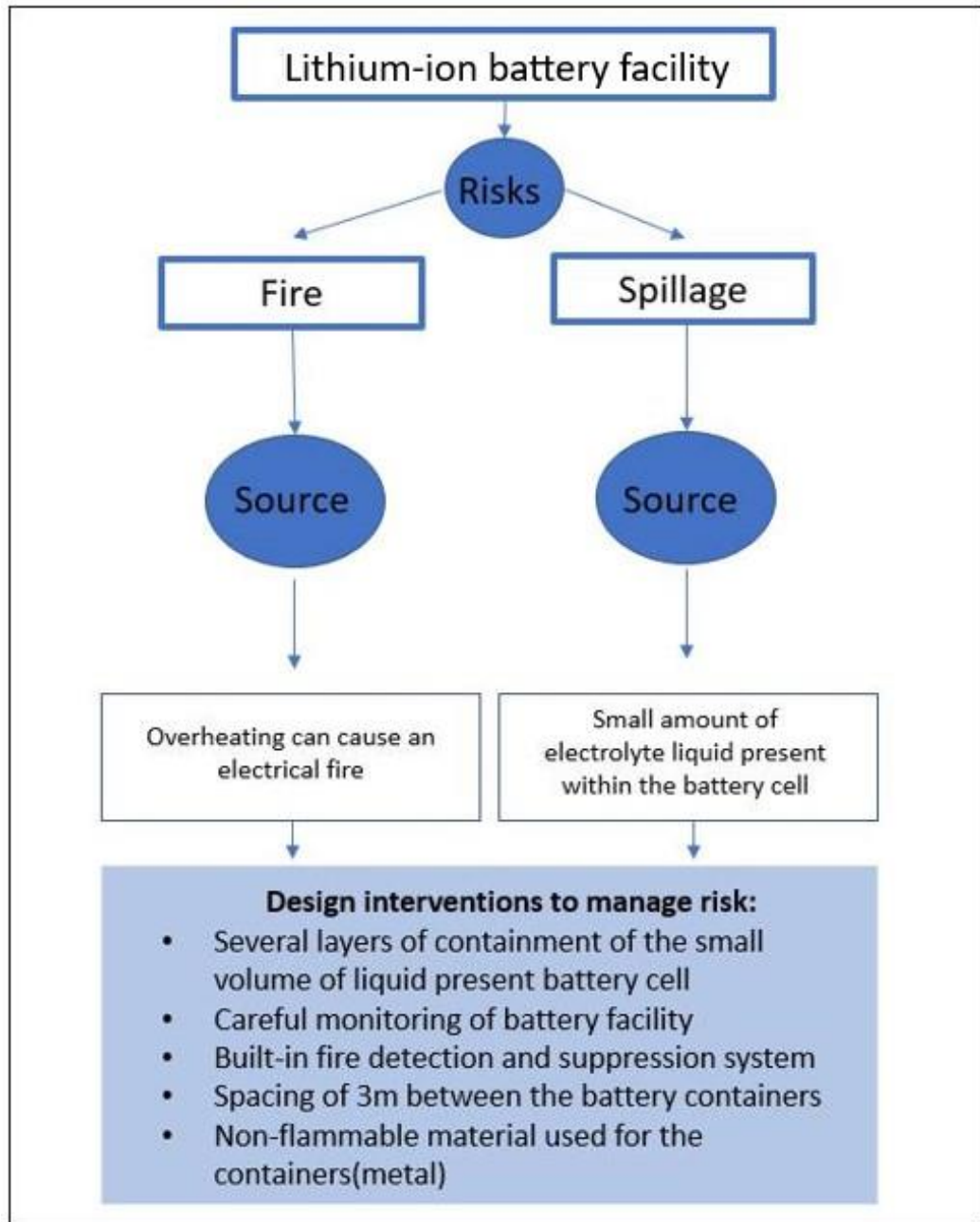
Figure 7-50 - Risk sources of the battery facility
