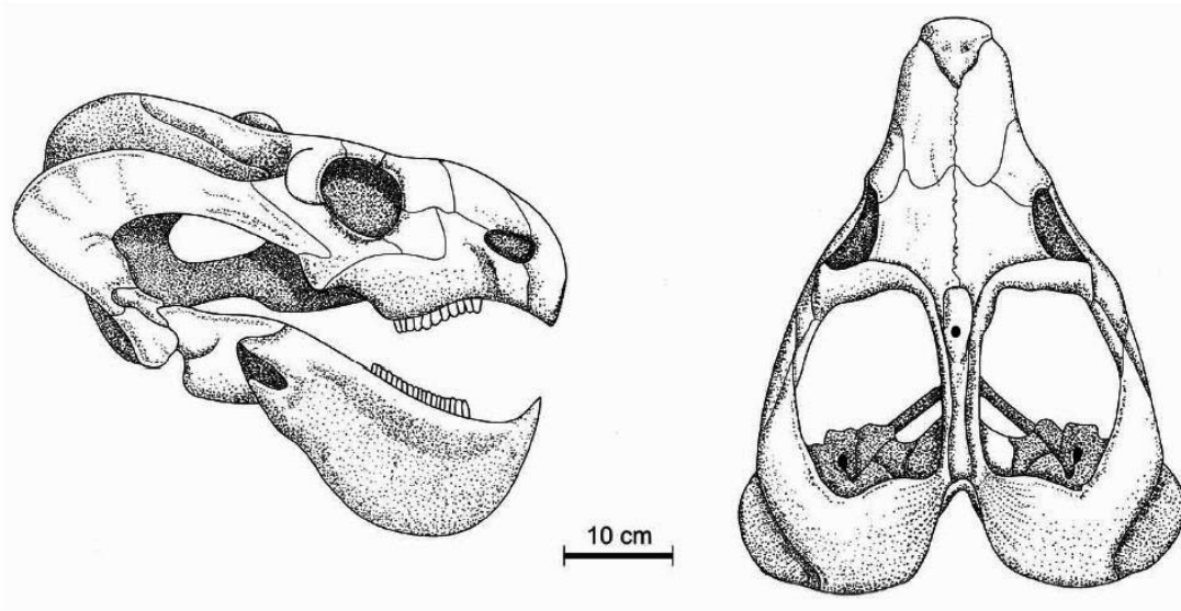
Figure 7-31 - Skull of the medium-sized dicynodont therapsid Endothiodon which occurs especially abundantly within the lower part of the Endothiodon Assemblage Zone
