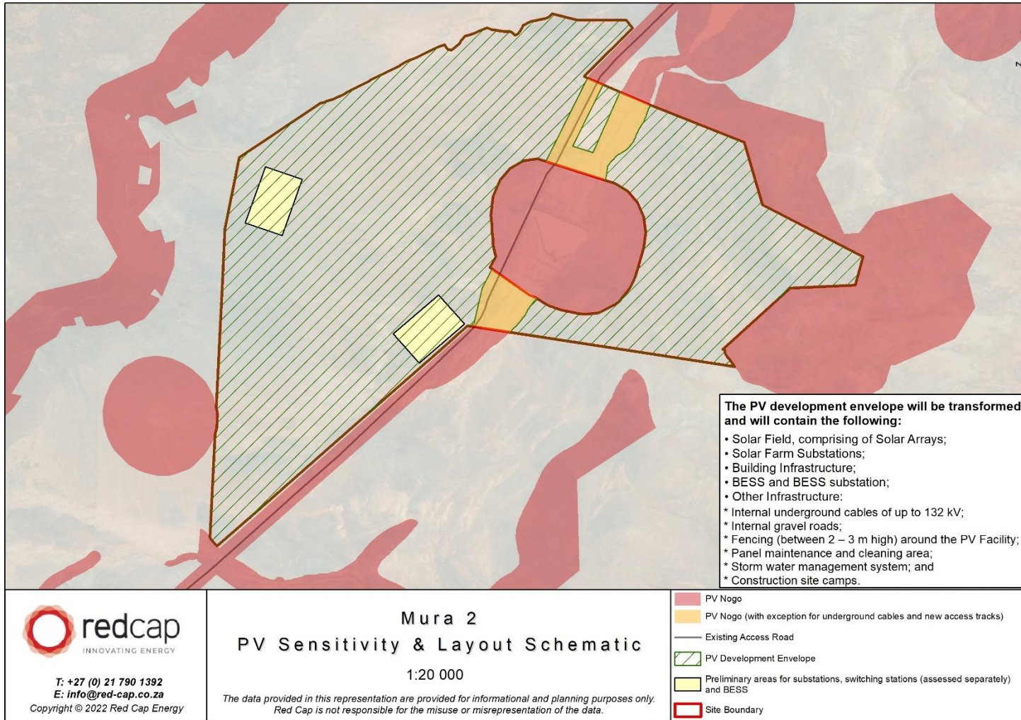
Figure 11-1 - Combined No-Go Sensitivity Map and Proposed Development Envelope for Mura 2 PV Facility
