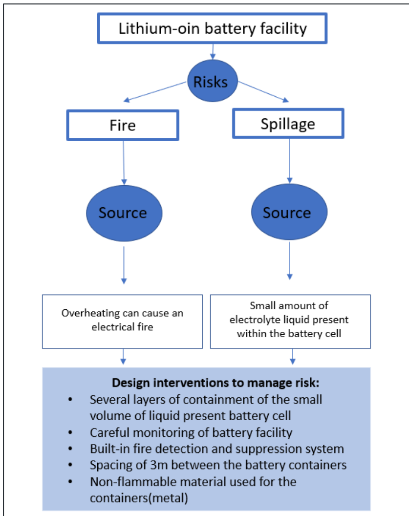
Figure 9-1 - Risk sources of the battery facility
