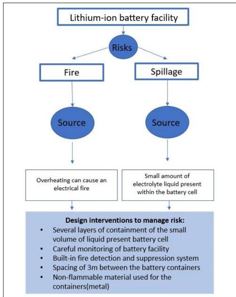
Figure 7-46 - Risk sources of the battery facility
