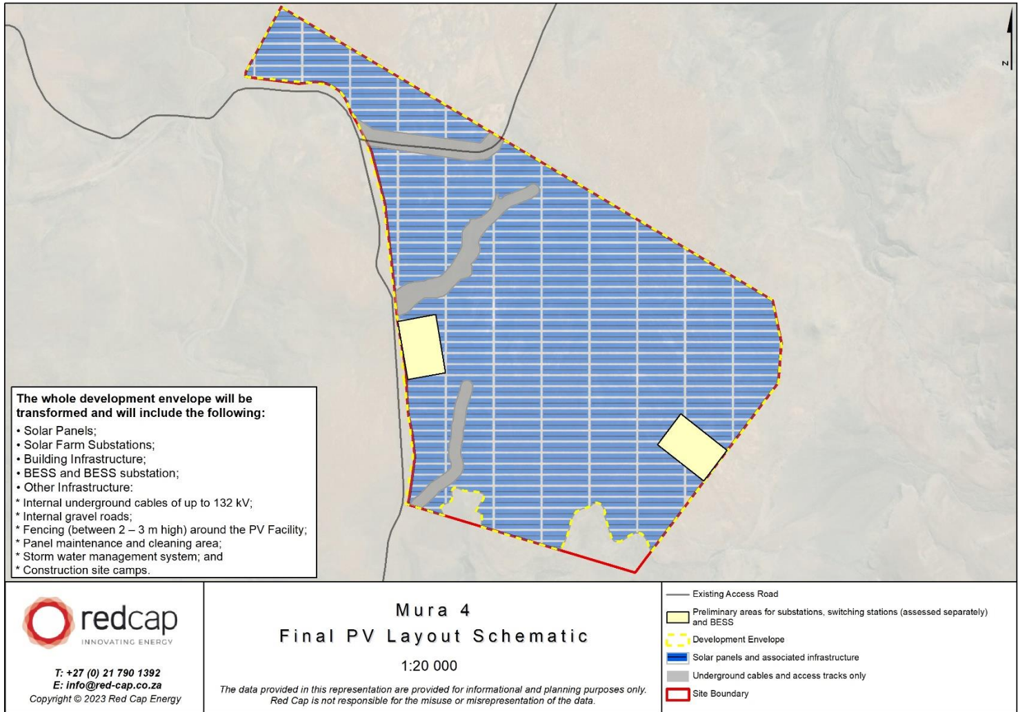
Figure 11-2 - Final Site Layout Map
