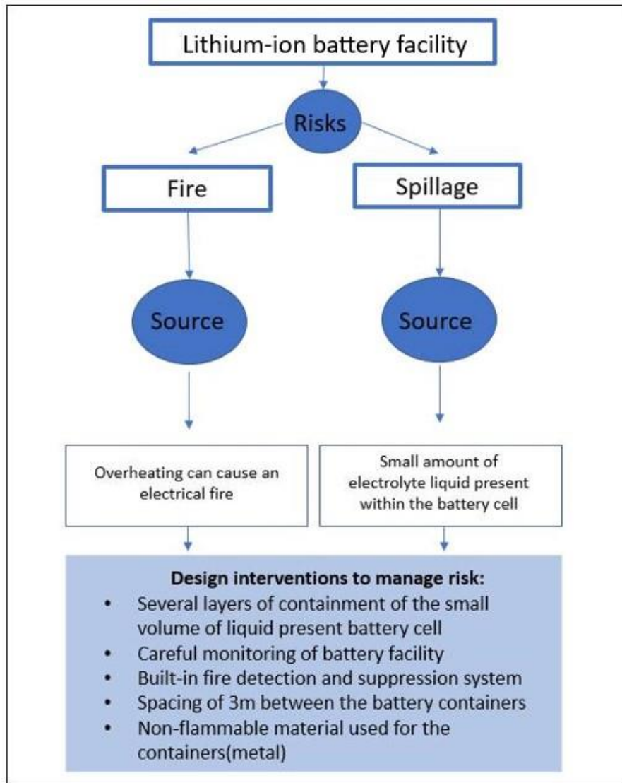
Figure 9-1 - Risk sources of the battery facility
