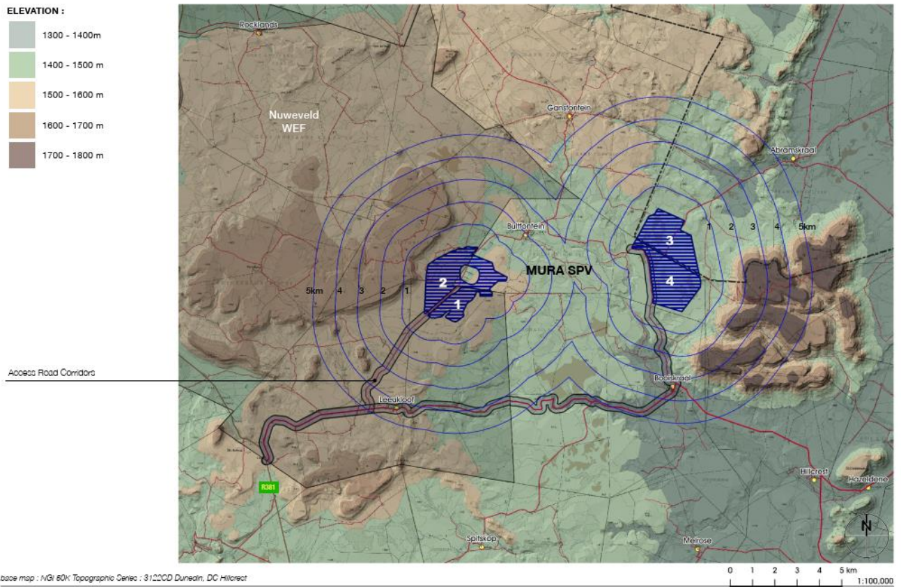
Figure 7-35 – Layout and Physiography
