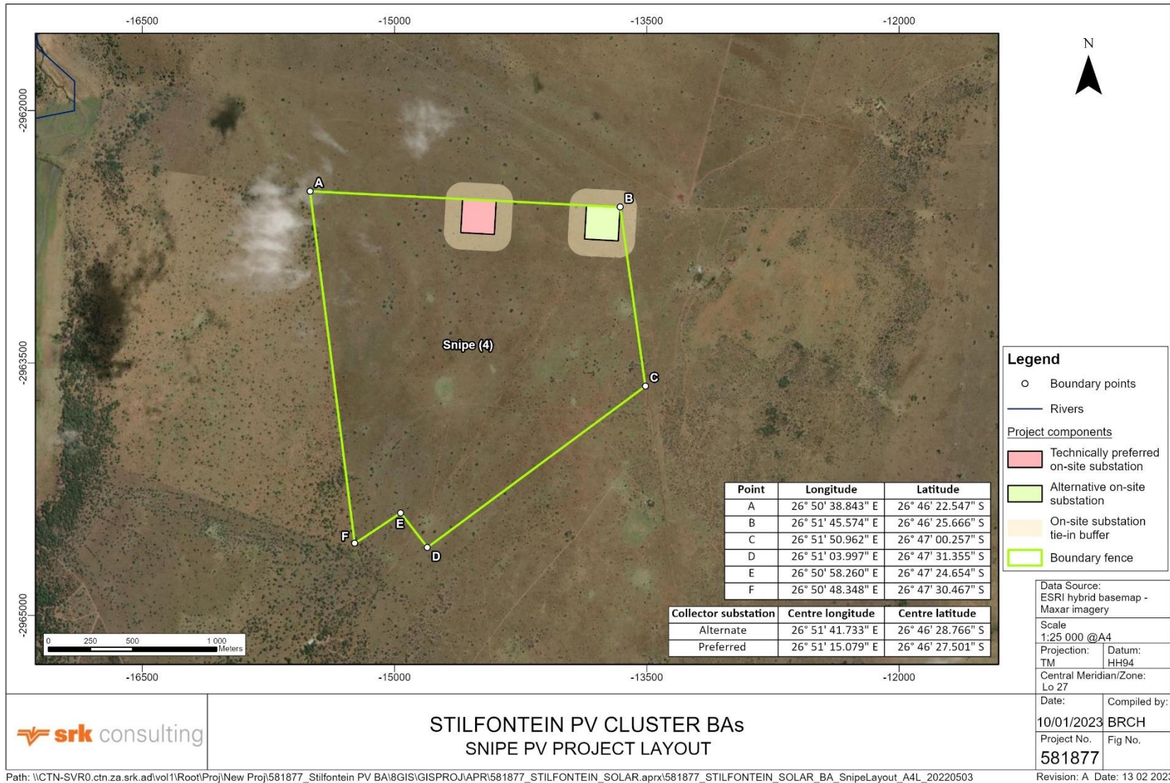
Figure 3-15: Layout of Snipe project
