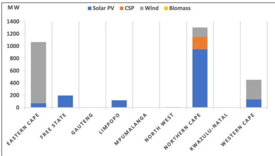
Figure 4-28: Distribution of renewable energy production in South African (2020)
