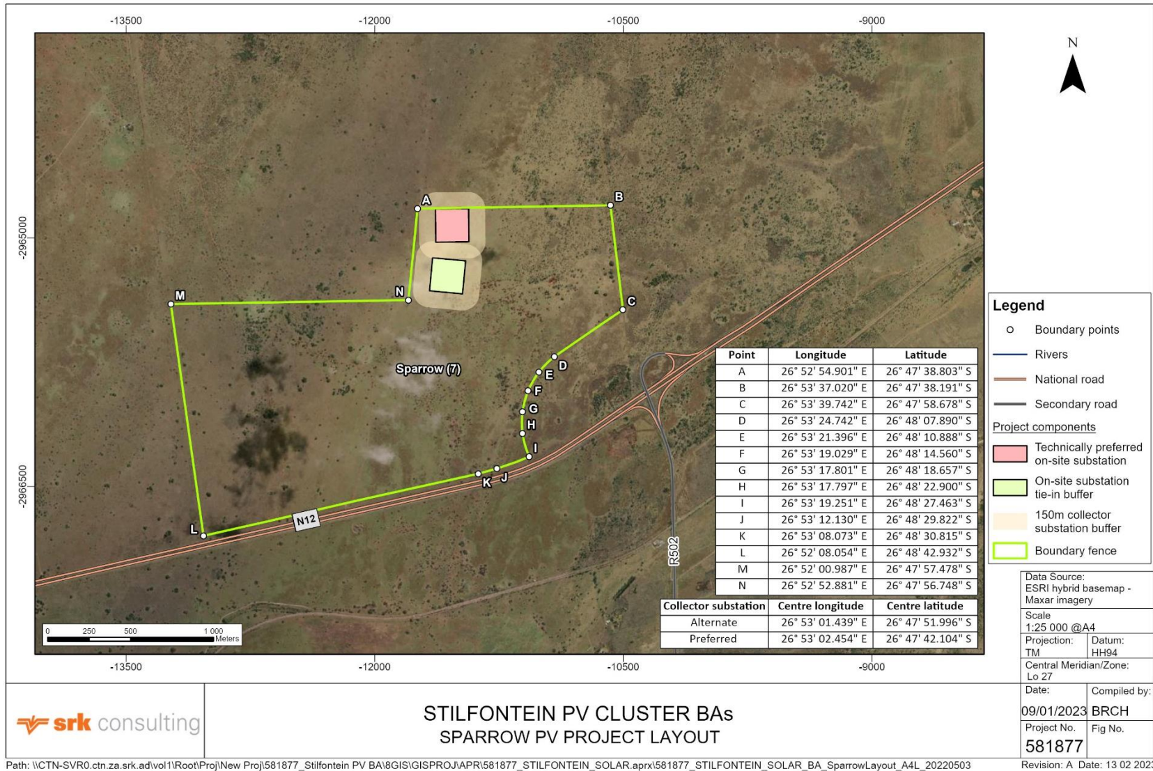
Figure 3-15: Layout of Sparrow project
