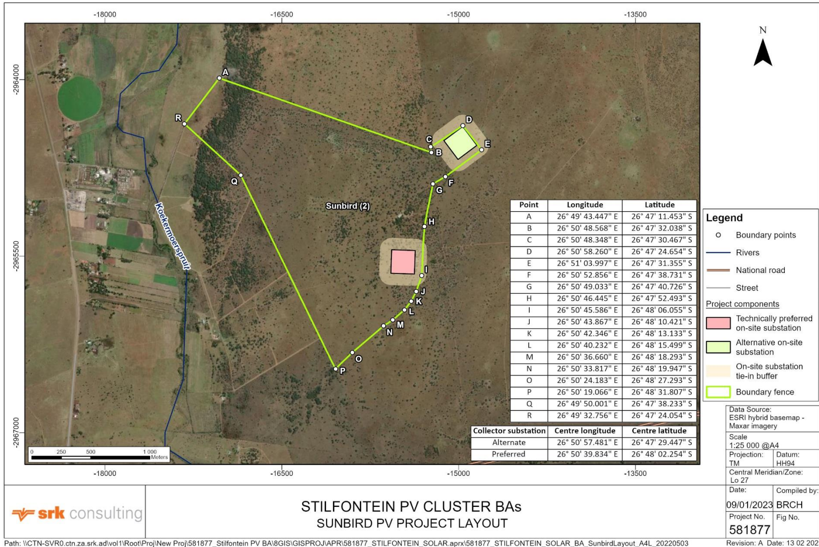
Figure 3-15: Layout of Sunbird project
