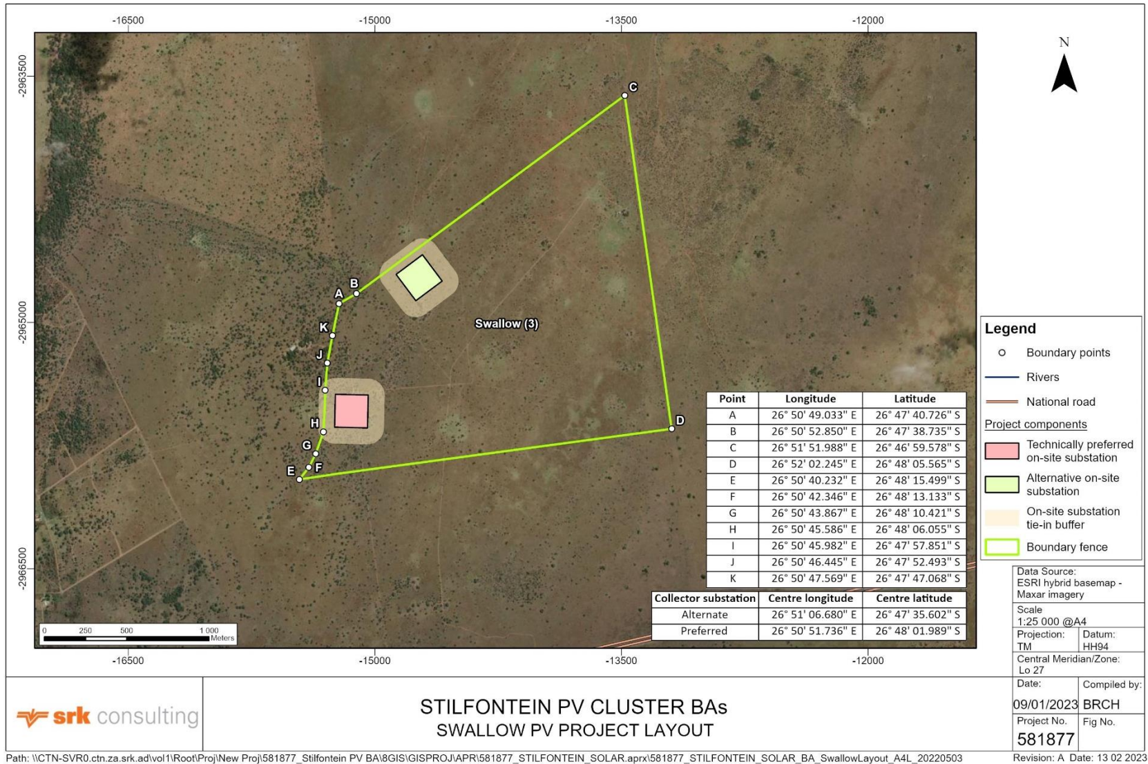
Figure 3-15: Layout of Swallow project
