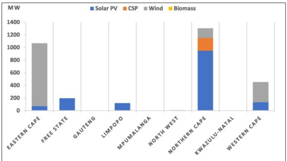
Figure 4-28: Distribution of renewable energy production in South African (2020)
