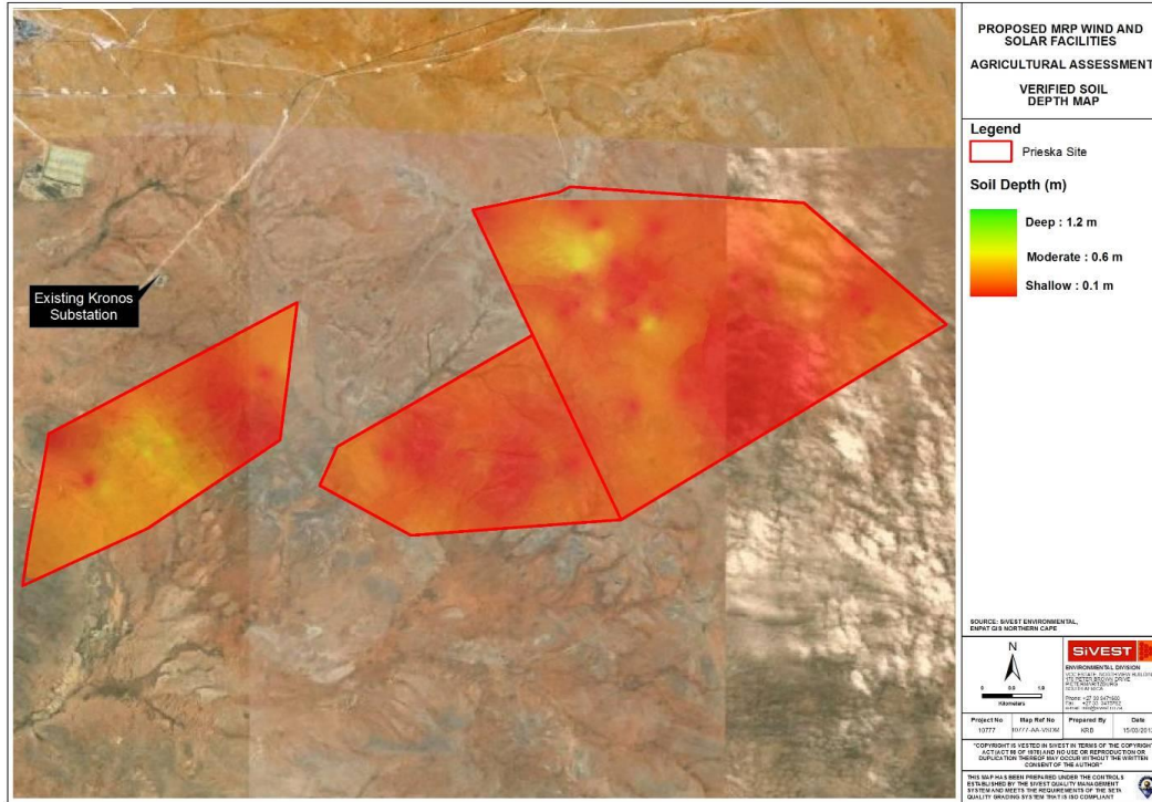
Figure 21: Verified Soil Depth Map
