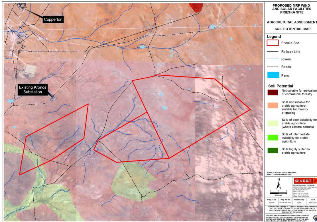
Figure 22: Soil Potential Map
