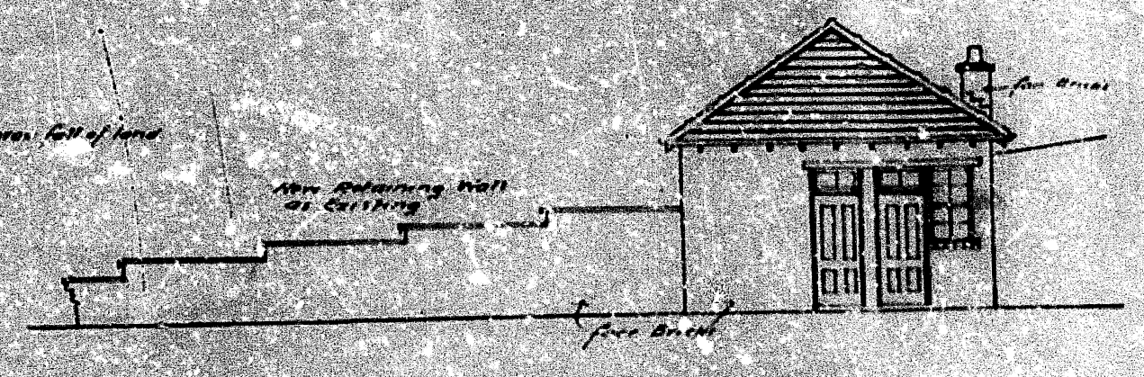
END ELEVATION TO PASSAGE
