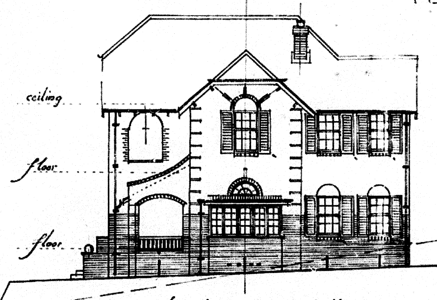
: Elevation to Sir Arthur Rd :
