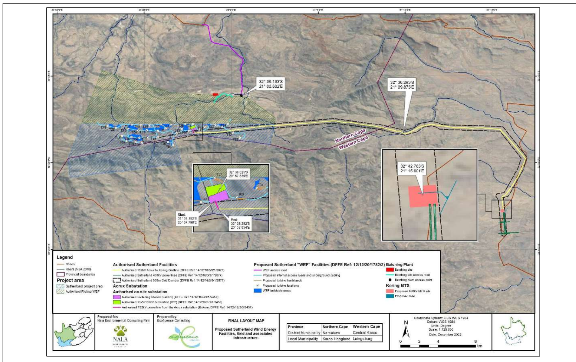
Figure 3: Final Layout Map of the Sutherland Wind Energy Facility and associated grid connection infrastructure.
