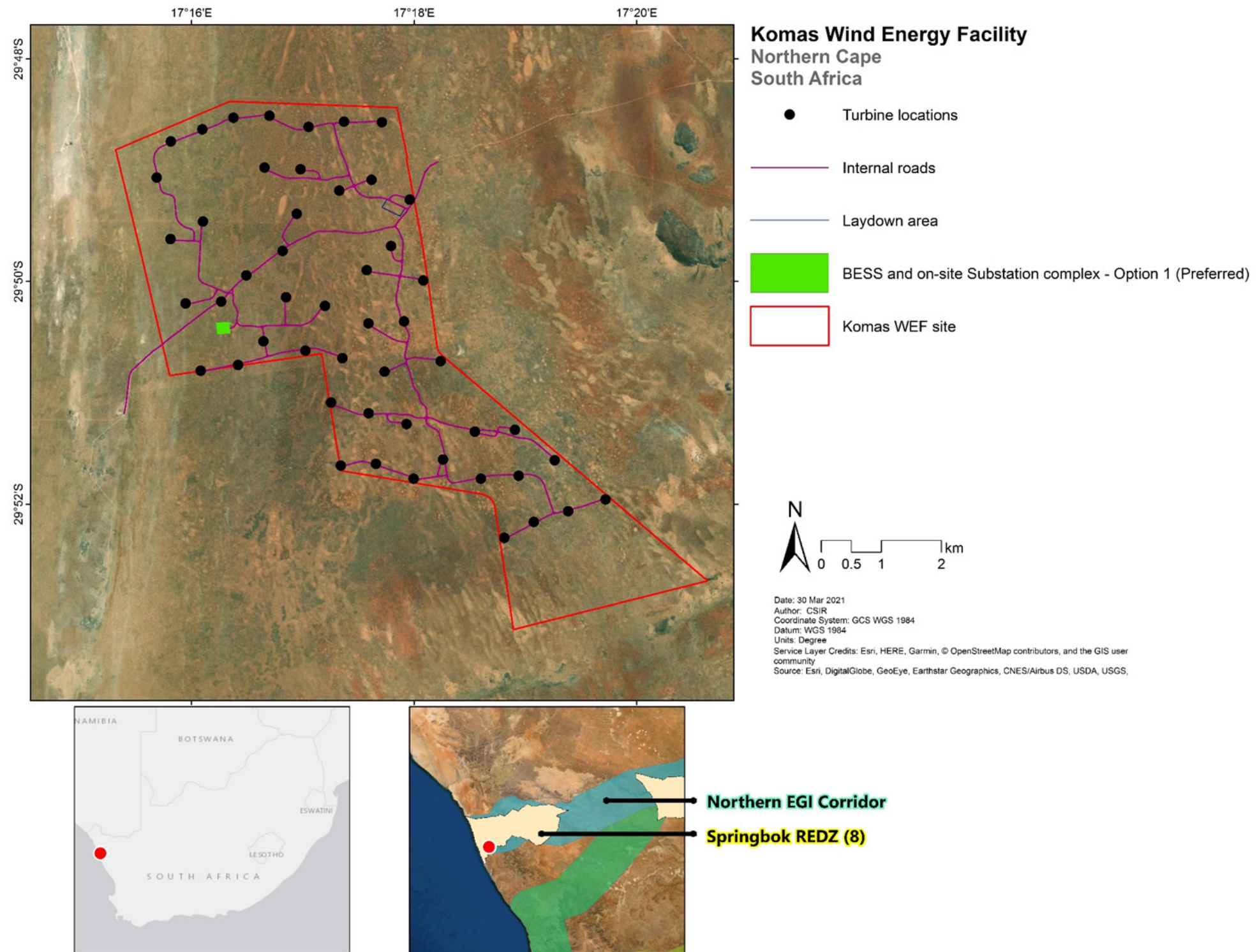
Appendix A.2: Preferred layout map of the proposed Komas Wind Energy Facility and associated infrastructure.
