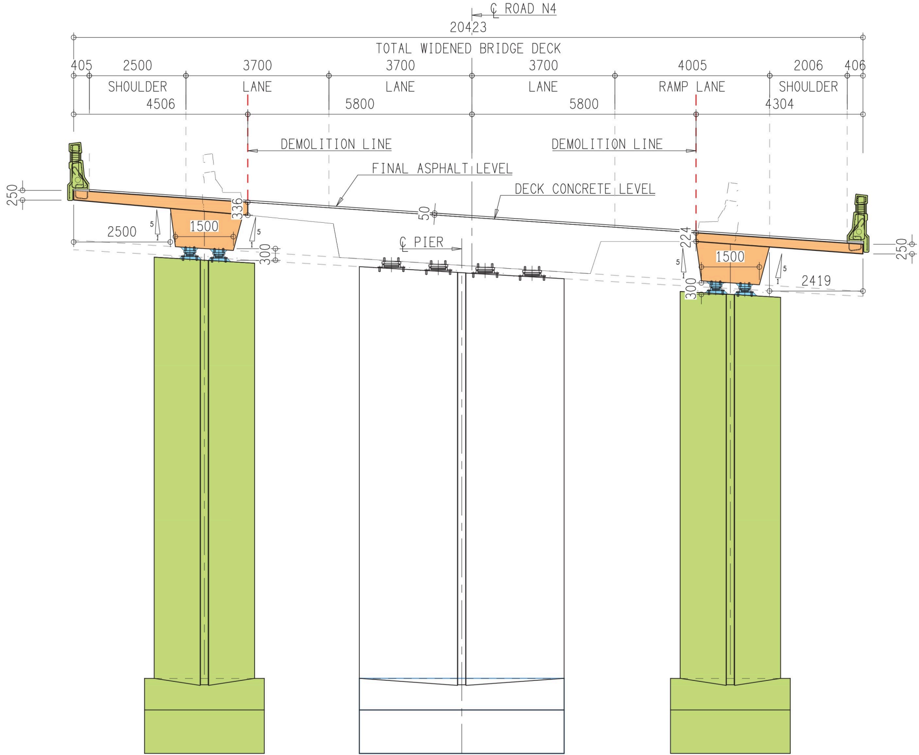
TYPICAL DECK CROSS SECTION AT PIER 2
