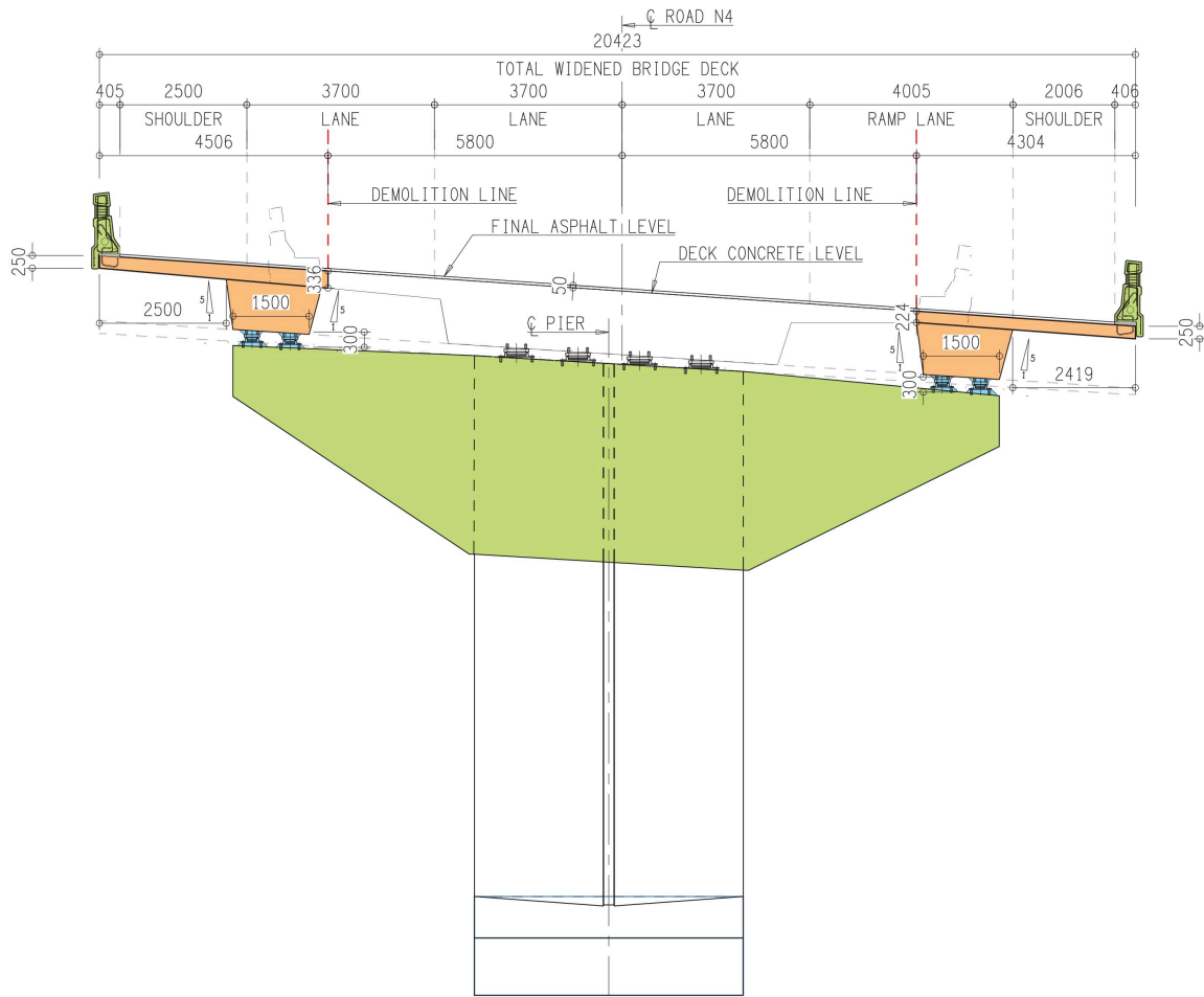
TYPICAL DECK CROSS SECTION AT PIER 2 SCALE 1:100
