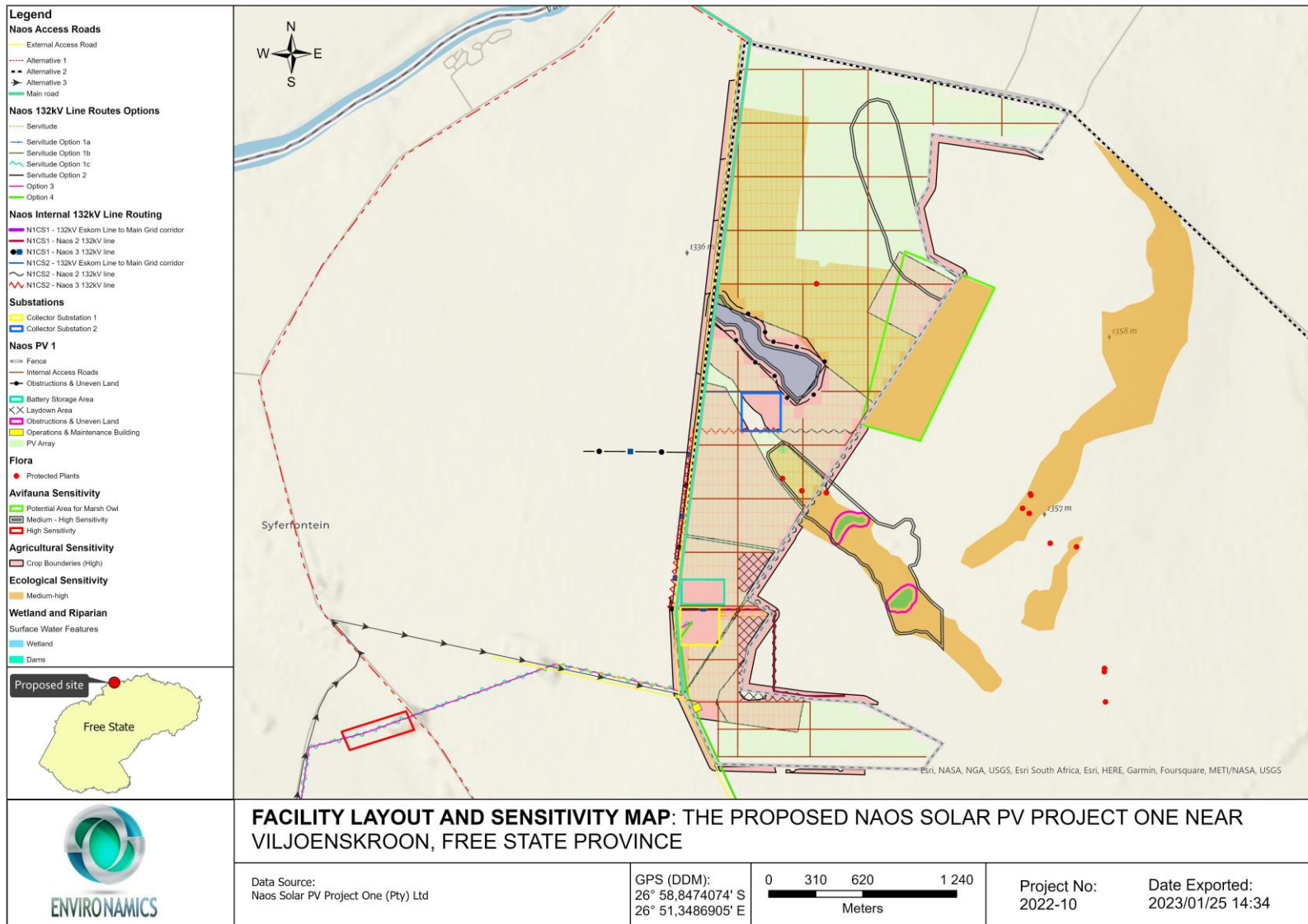
Figure 1: Environmental sensitivity map of the Naos Solar PV Project One – solar energy facility
