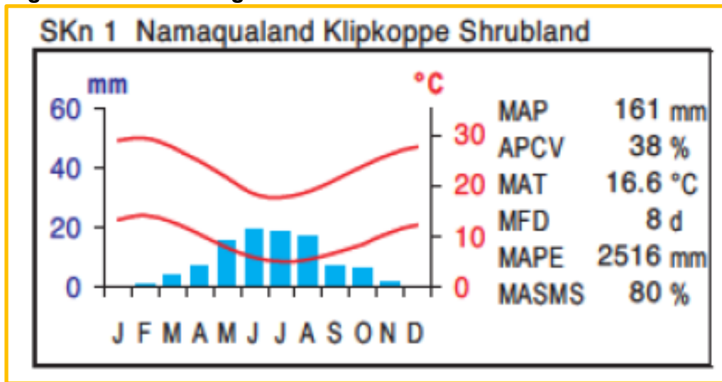
Figure 8: Climate diagram
