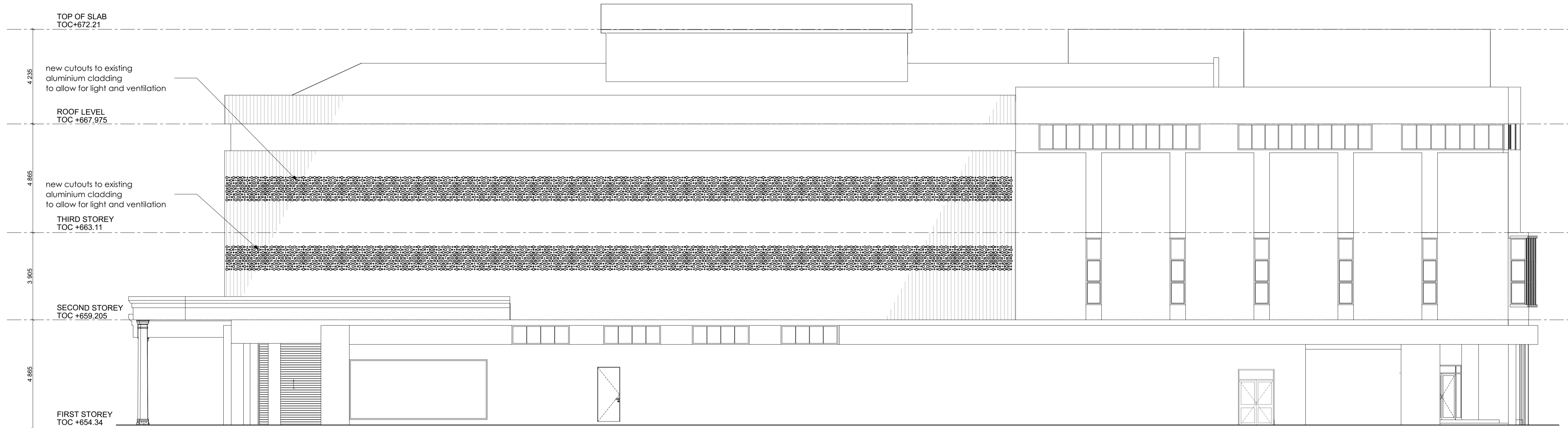
SOUTH WEST ELEVATION 1:100
