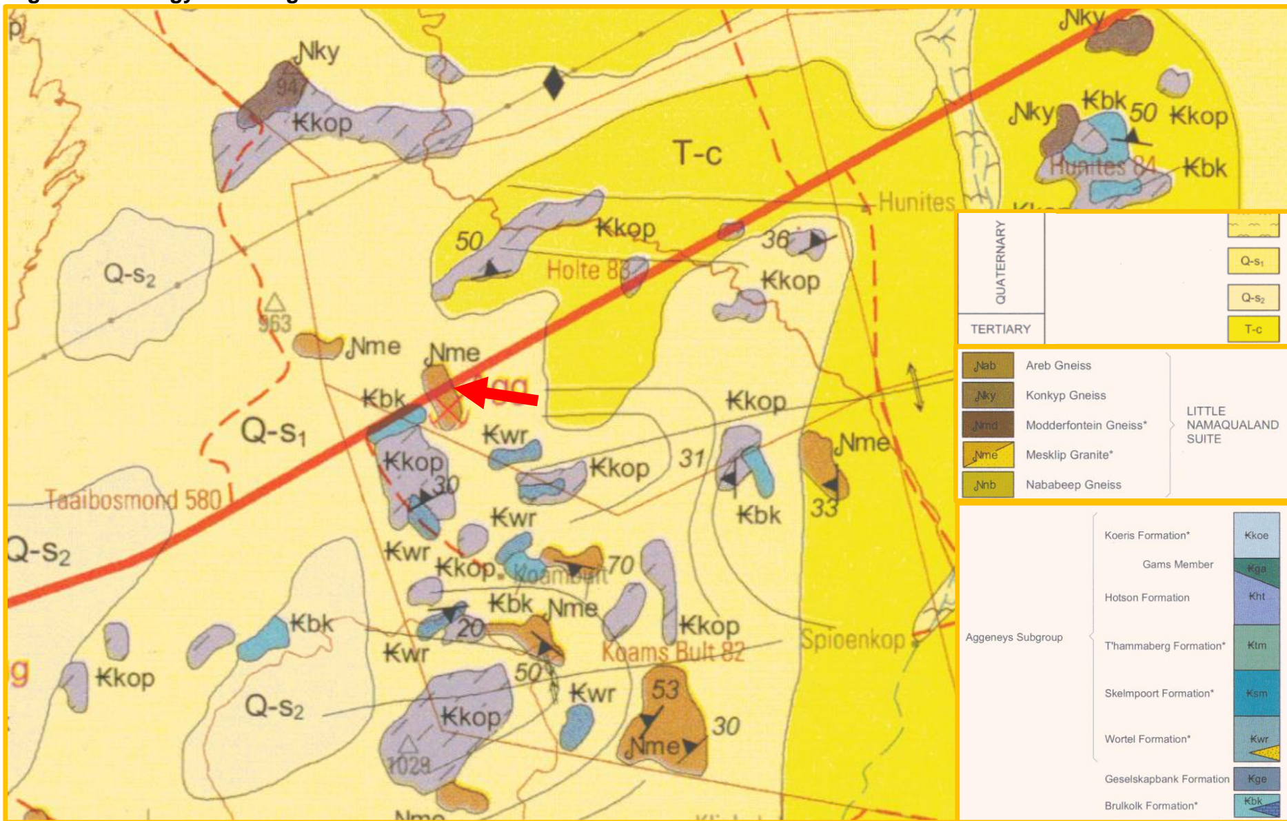
Figure 6: Geology of Mining area
