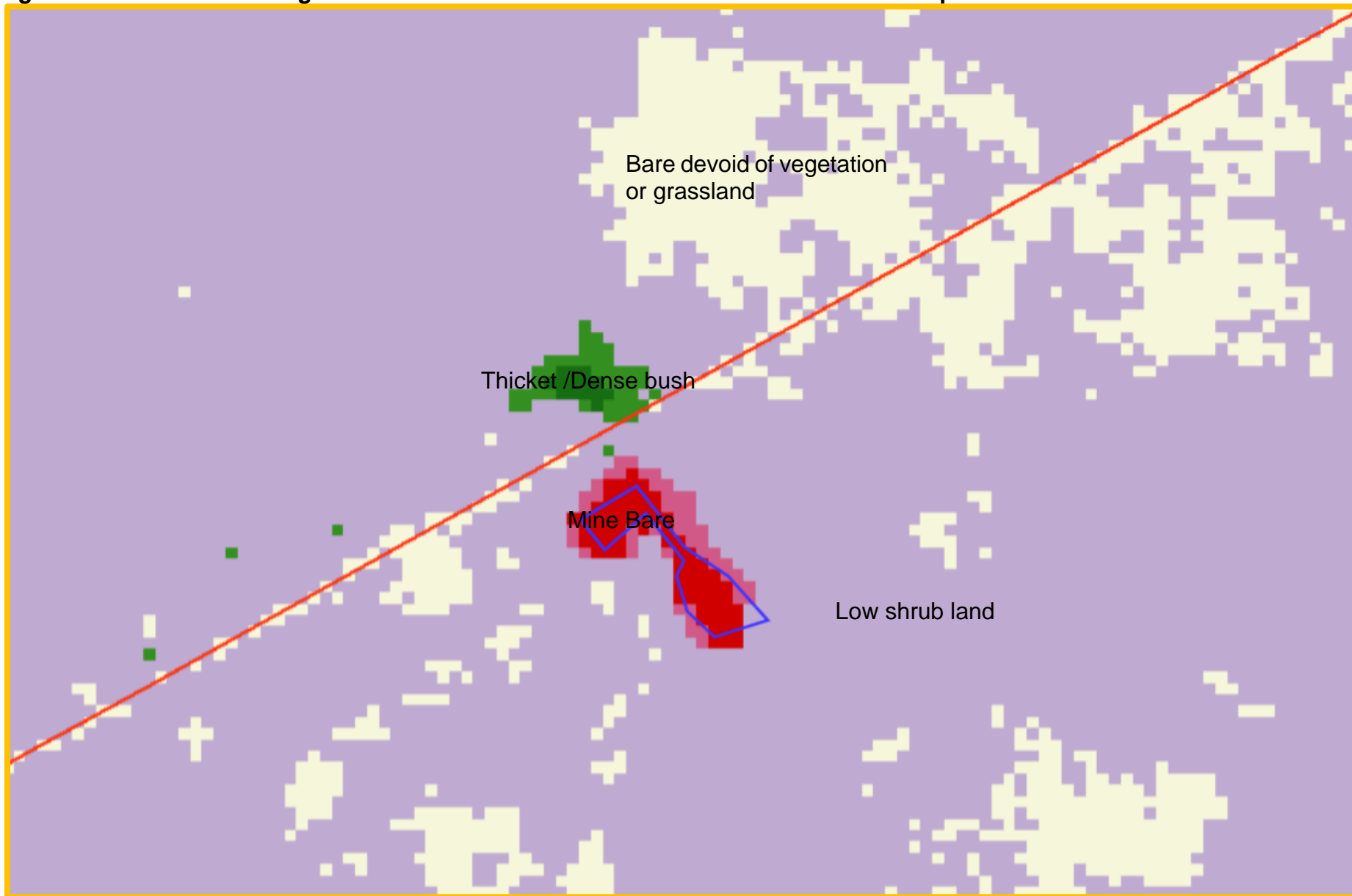
Figure 7: Location of Mining area in terms of Land Cover sourced off SANB BGIS Map Viewer
