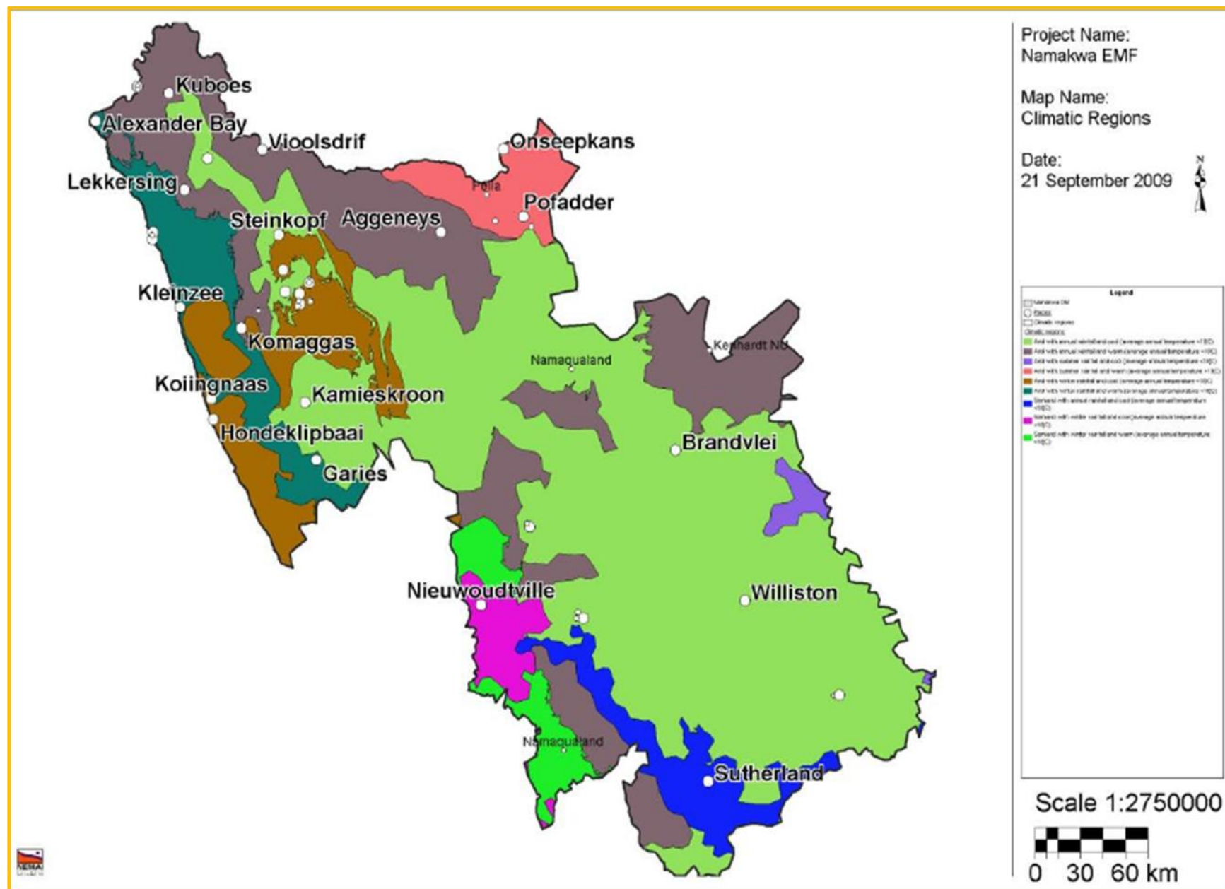
Figure 9: Climate (Climatic regions within the NDM)
