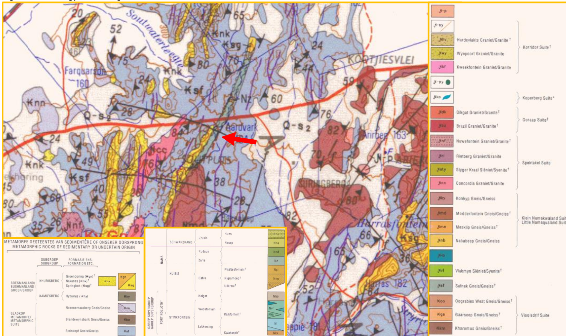
Figure 6: Geology of Mining area
