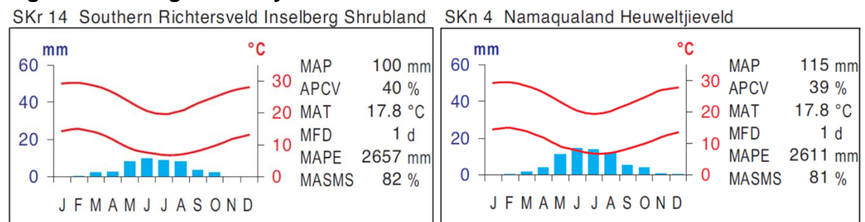
Figure 8: Average monthly rainfall
