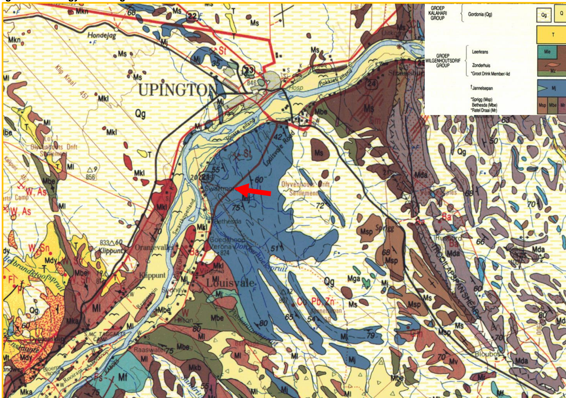
Figure 6: Geology of Mining area
