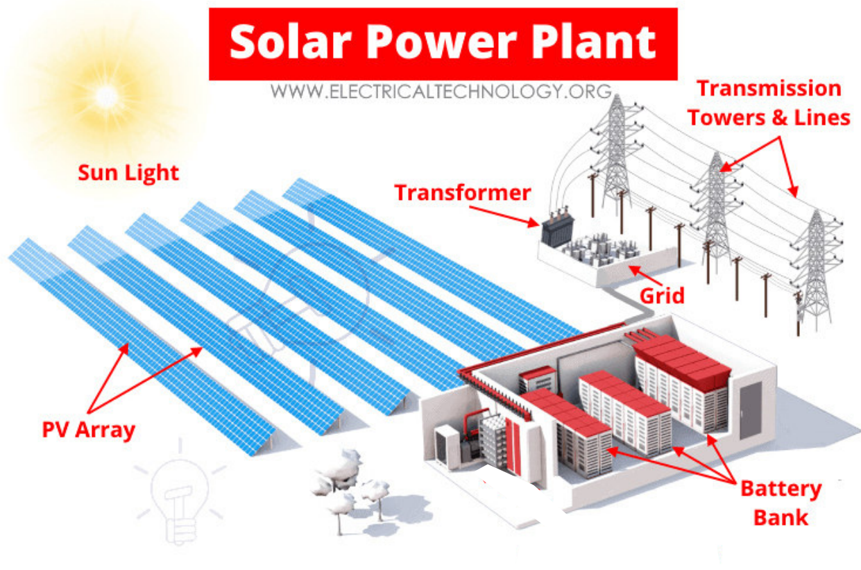
Figure 2-2: Simplified diagram of the main components of a Solar Facility. (Source: https://www.electricaltechnology.org ).
