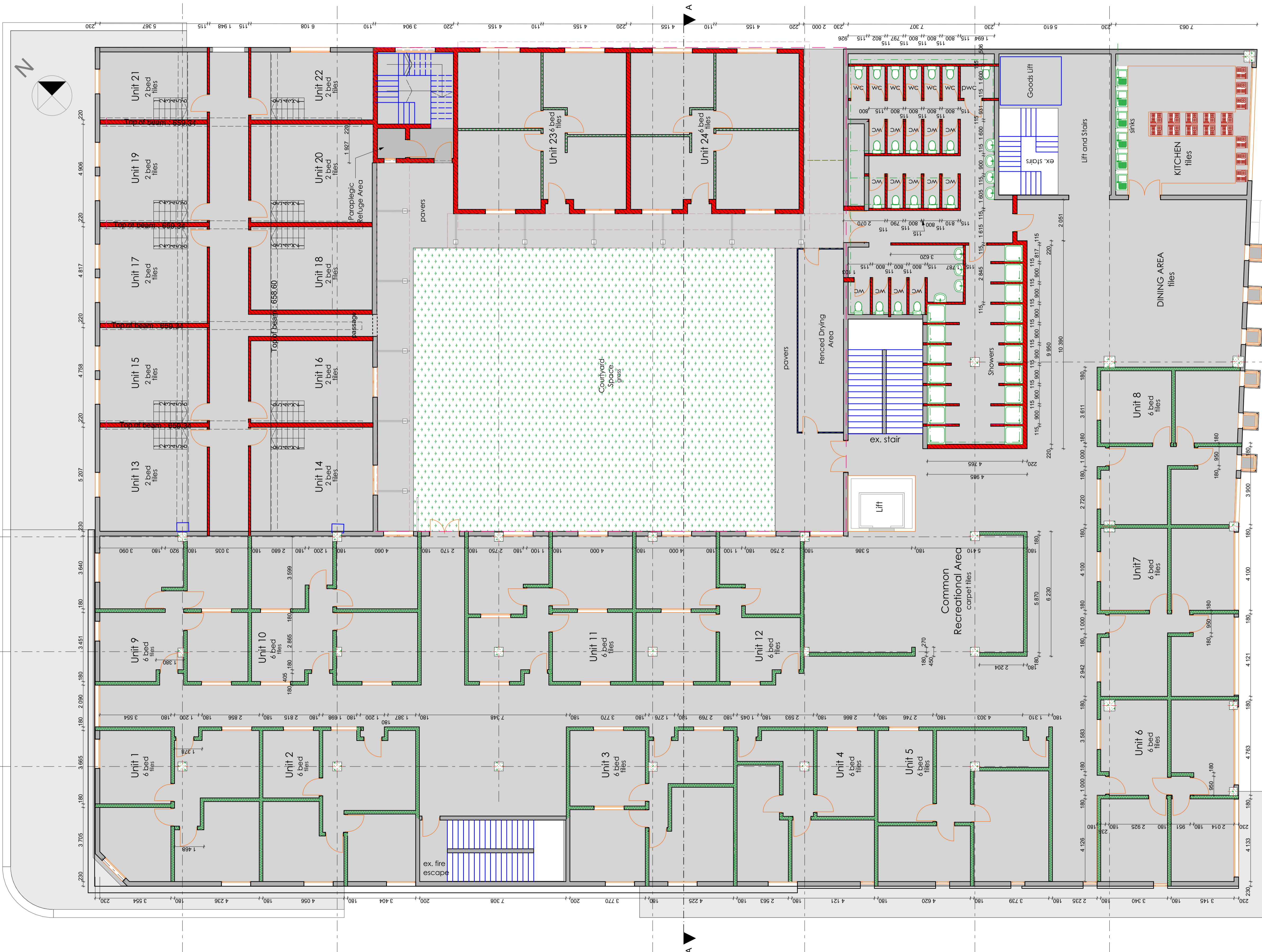
First Floor 1:100
