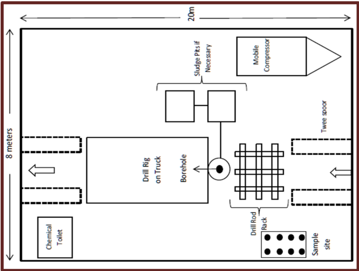
Figure 3 Typical layout of a diamond drill platform
