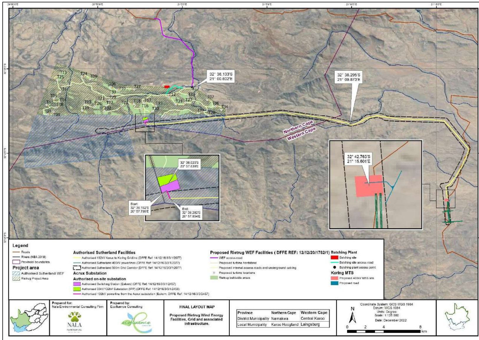
Figure 1.1. Authorized 140MW Rietrug Wind Energy Facility (WEF) and Grid Connection Infrastructure Layout
