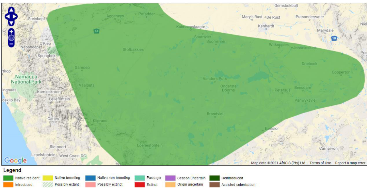
Figure 5-4: Red lark ( Calendulauda burra ) distribution map (BirdLife International, 2021 b ).
