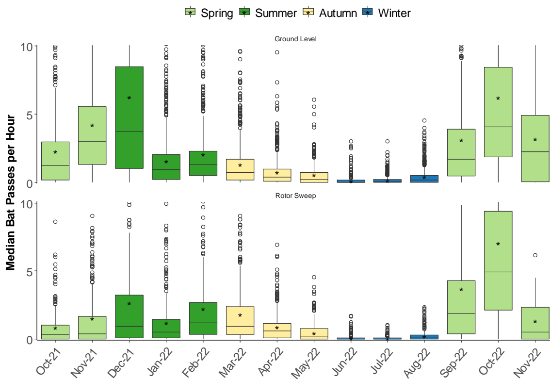
Graph 1: Boxplot showing the temporal distribution of median bat passes per detector per hour per month.
