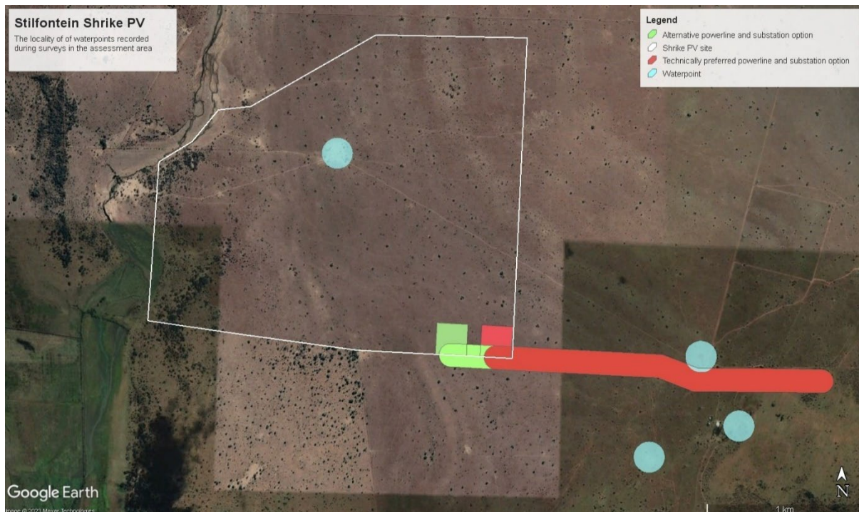
Figure D1: Shrike PV sensitivities map showing waterpoints, powerline options and on-site substation options.
