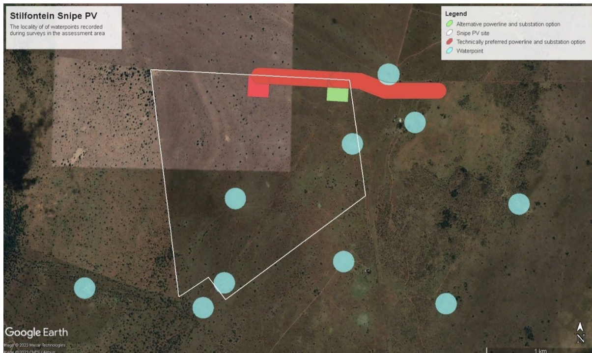
Figure D1: Snipe PV sensitivities map showing waterpoints, powerline options and on-site substation options.
