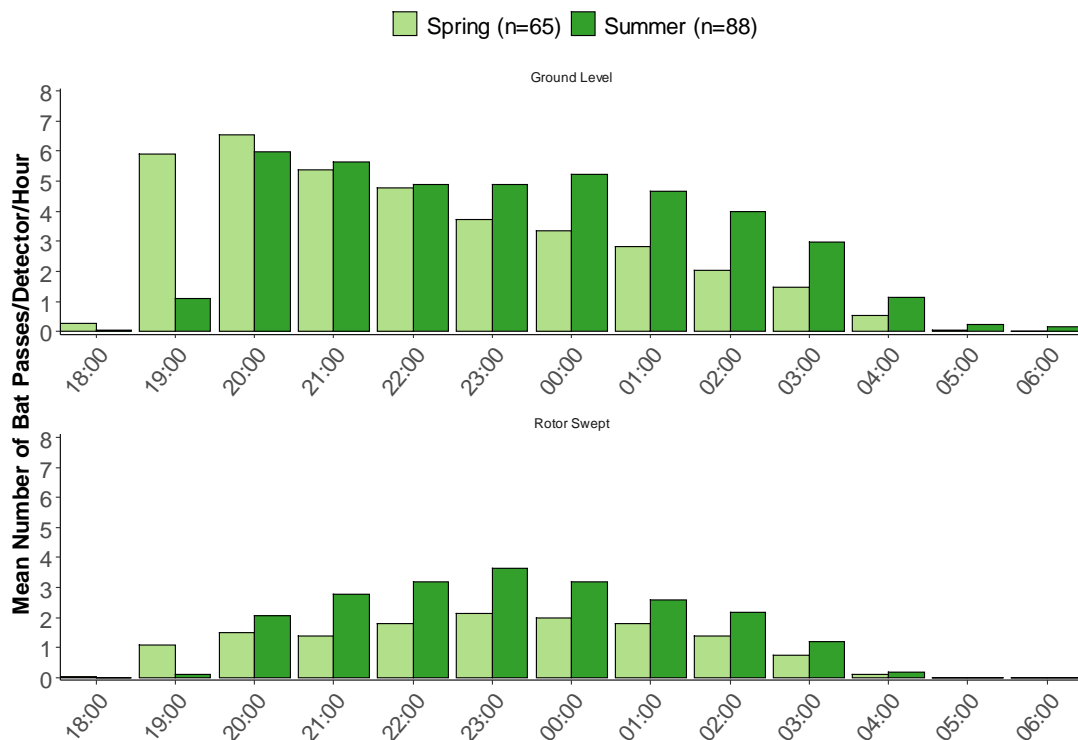
Graph 3: Bar graph showing the mean number of bat passes per detector per hour at Ground Level and Rotor Sweep.
