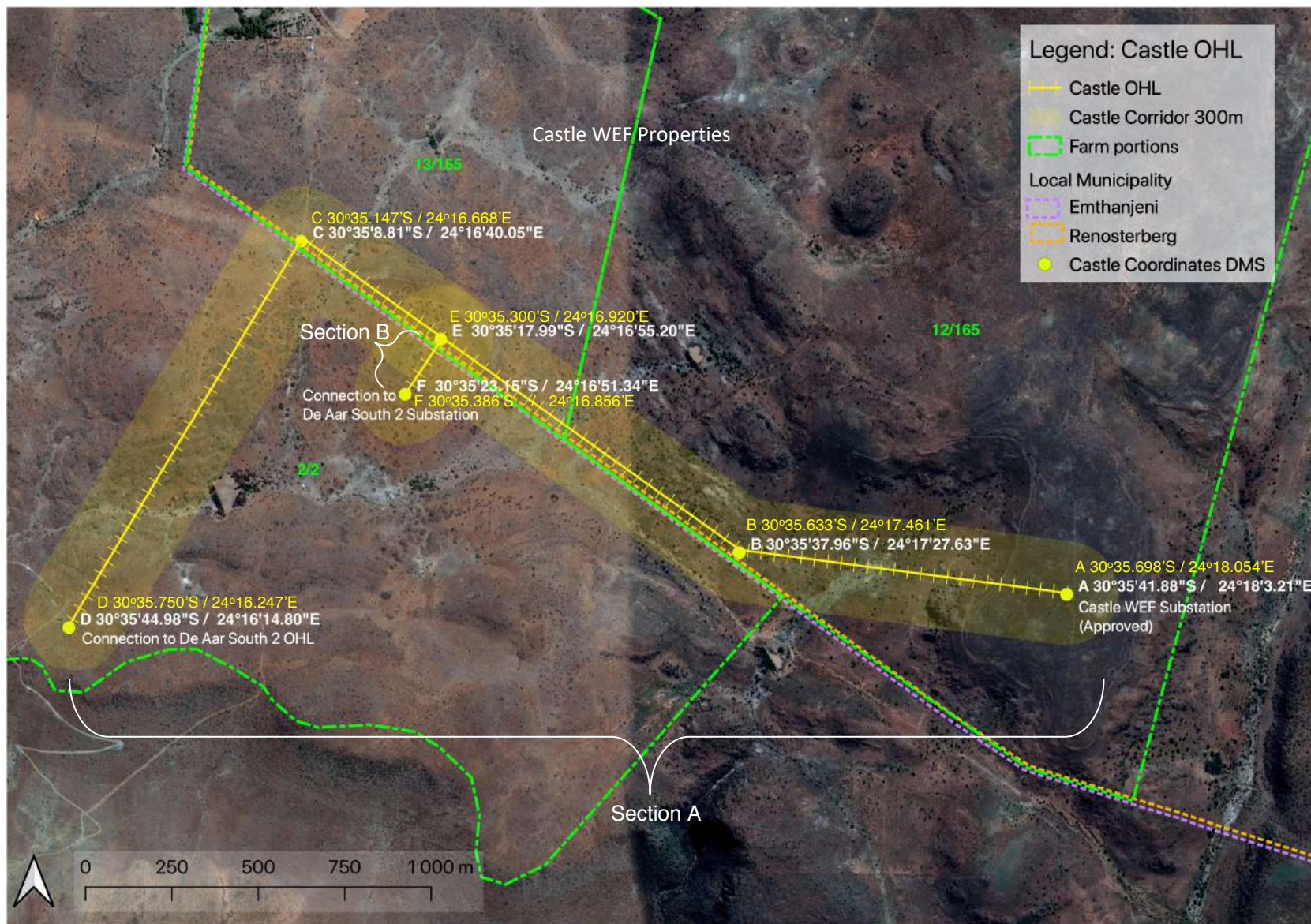
Figure 1: Layout of the proposed Castle OHL near De Aar in the Northern Cape Province (Satellite image).
