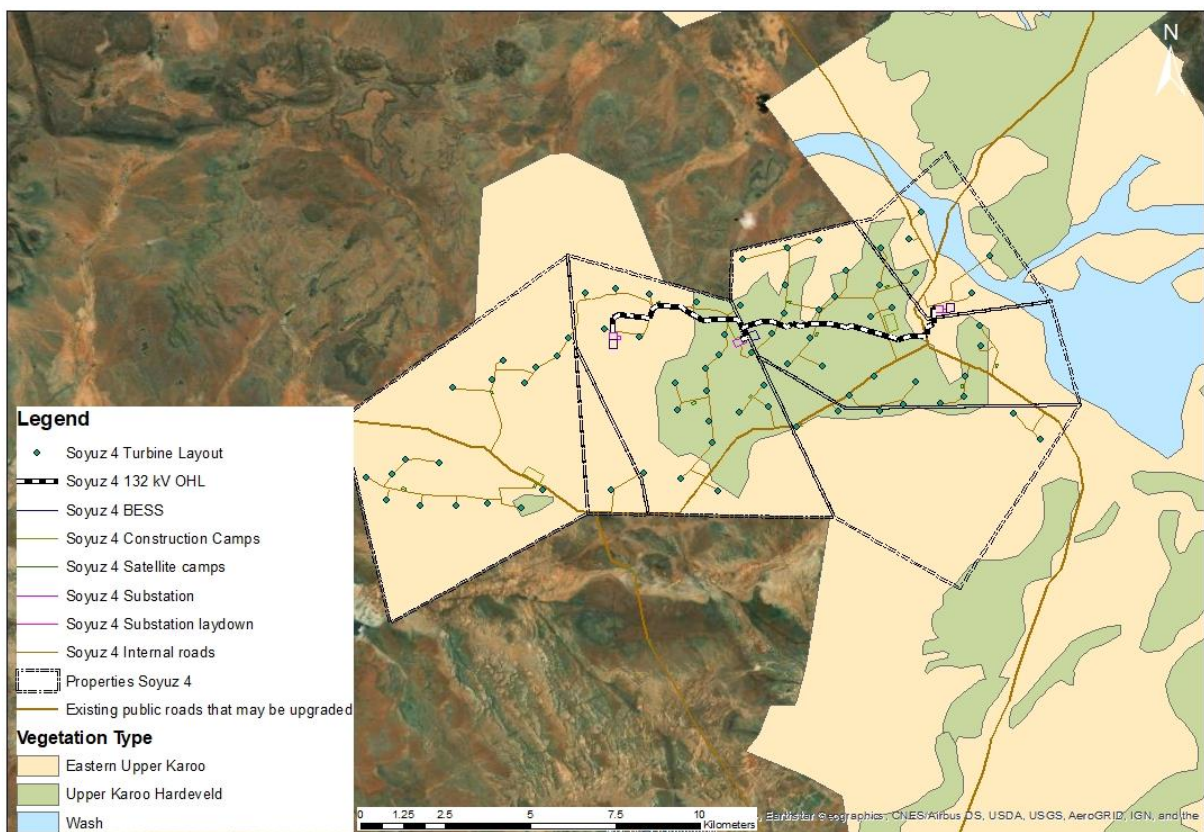
Figure 3.1: Vegetation map for the project site (Botanical Scoping Report, Biodiversity Africa, 2023)
