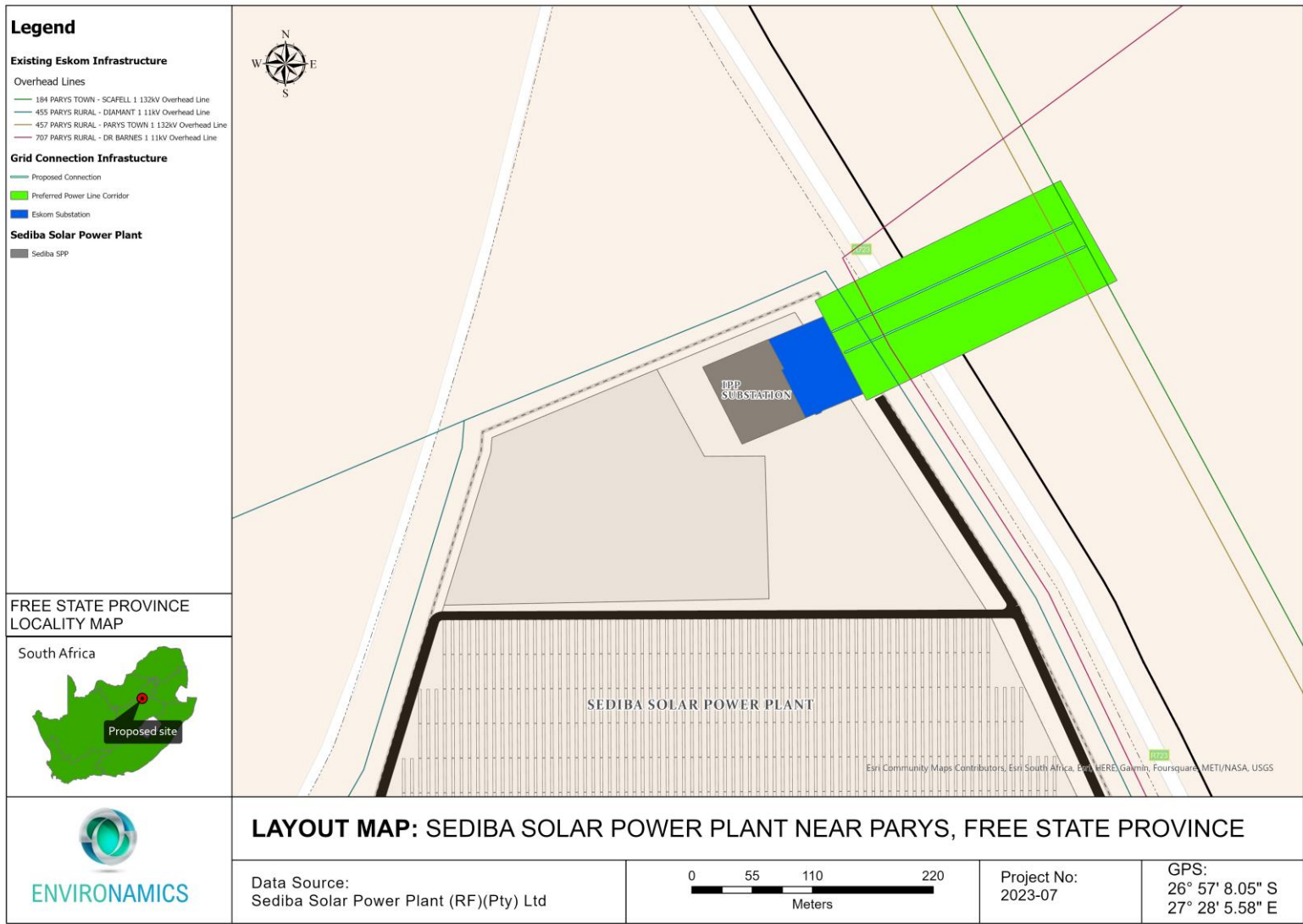
Figure 2: Layout map of the Sediba Solar Power Plant illustrating the location of the portion of the substation that will belong to Eskom authorised for the Sediba Solar Power Plant.
