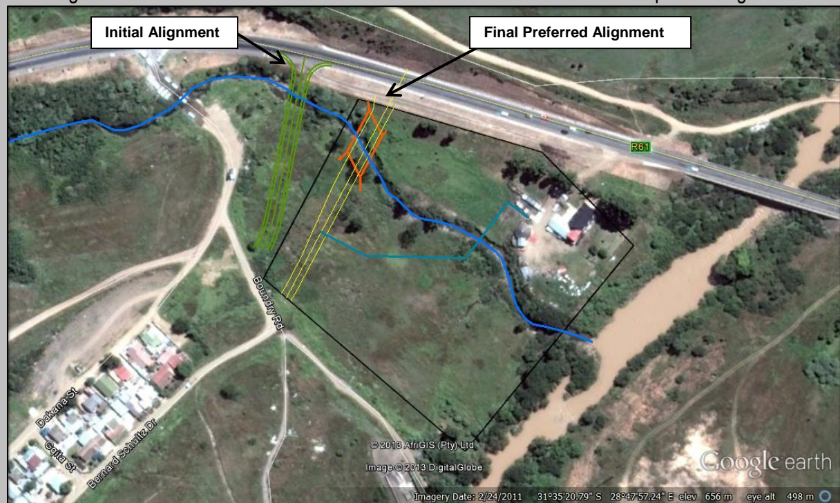
Figure 3: Alignment Alternatives Considered
