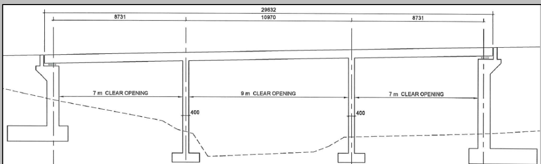
Figure 6: Bridge Design Option C
