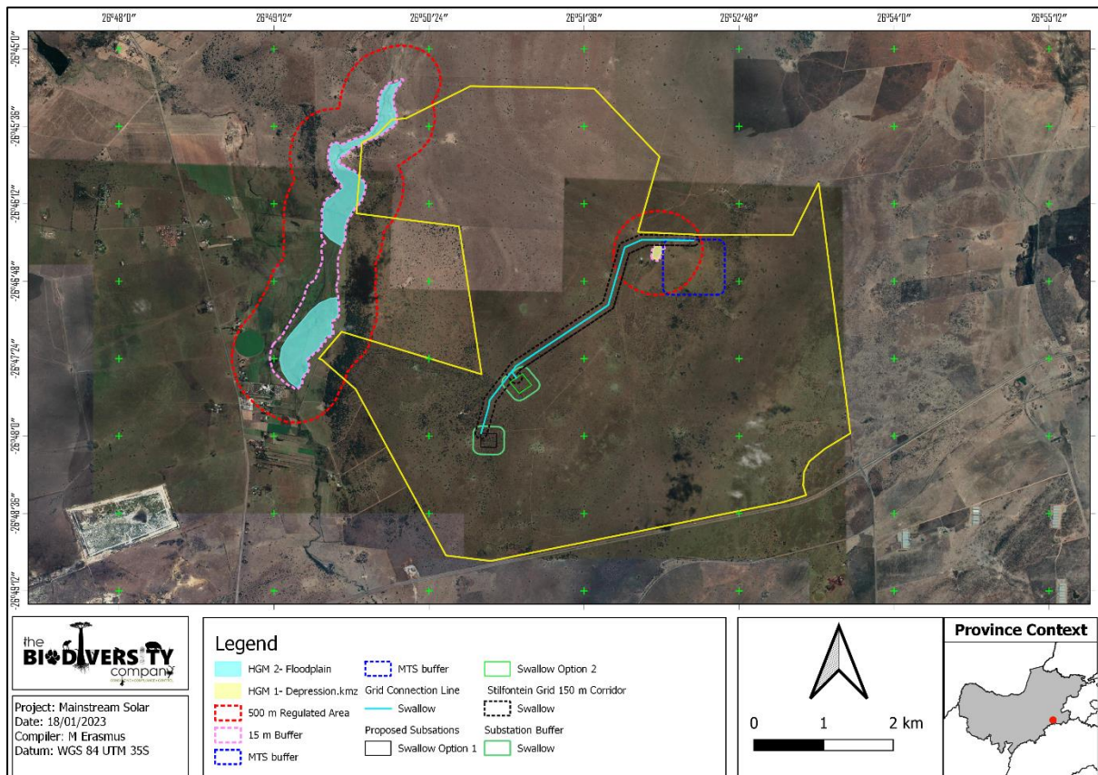
Figure 10-1 Location of the Swallow grid infrastructure with relation to the Stilfontein cluster project area as well as the delineated wetlands inside the cluster area.
