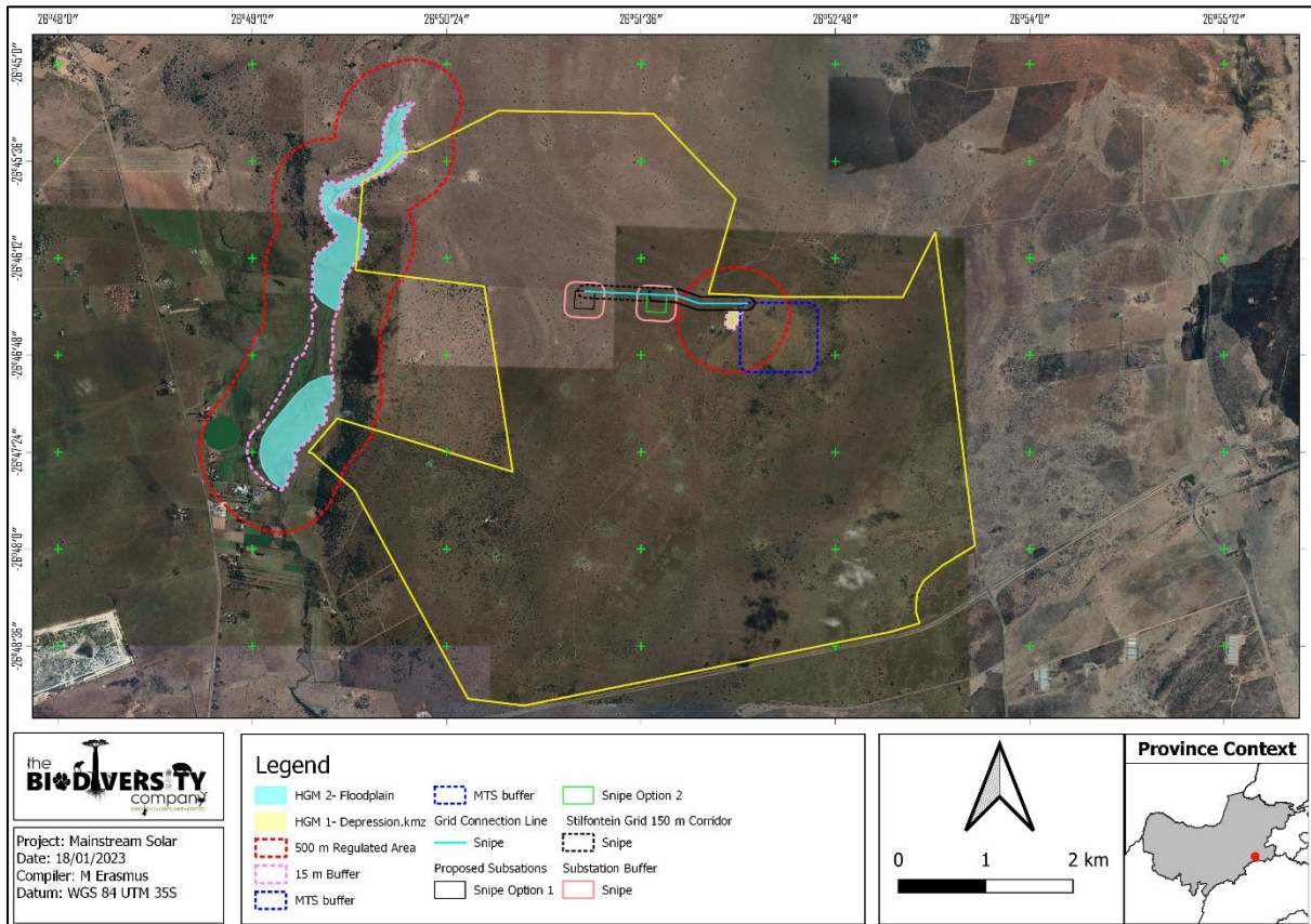
Figure 10-1 Location of the Snipe PV grid infrastructure with relation to the Stilfontein cluster project area as well as the delineated wetlands inside the cluster area.
