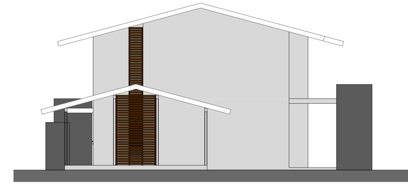
west elevation 1:100
