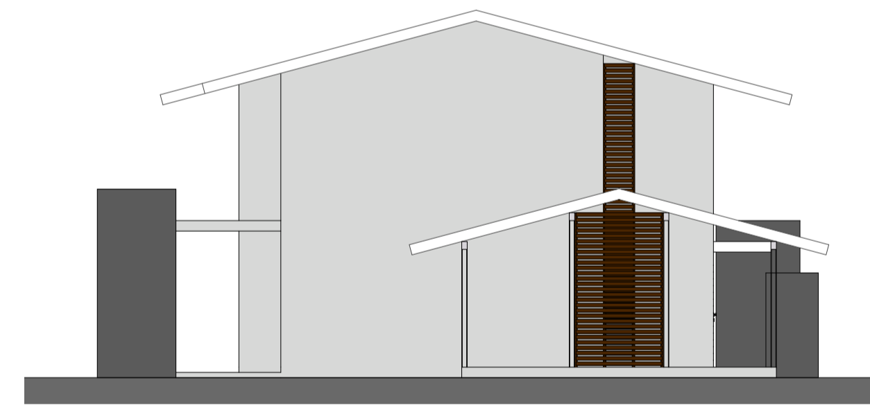
east elevation 1:100
