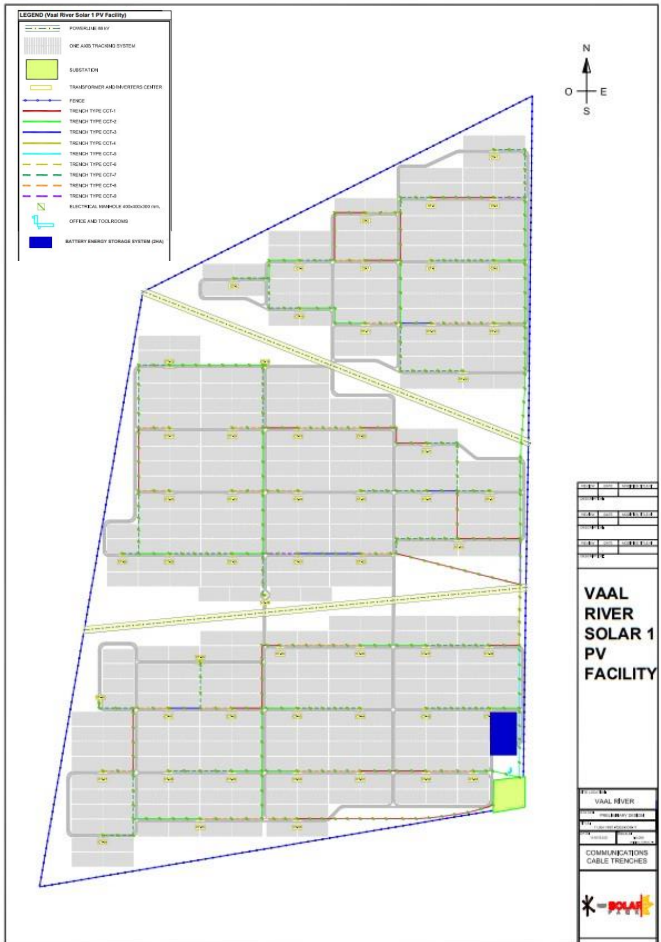
Figure 3.2: Map showing the layout of the BESS within the authorised development footprint of the solar PV facility
