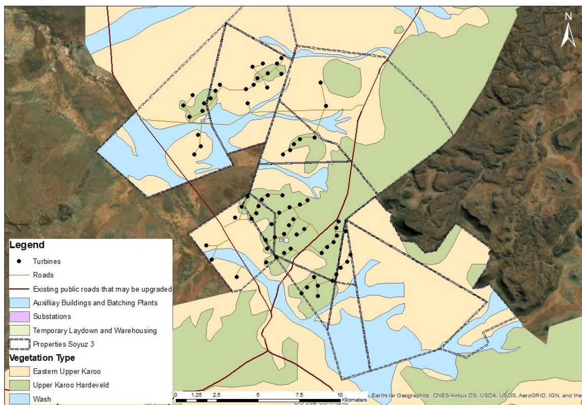
Figure 3.1: Vegetation map for the project (Botanical Scoping Report, Biodiversity Africa, 2020)
