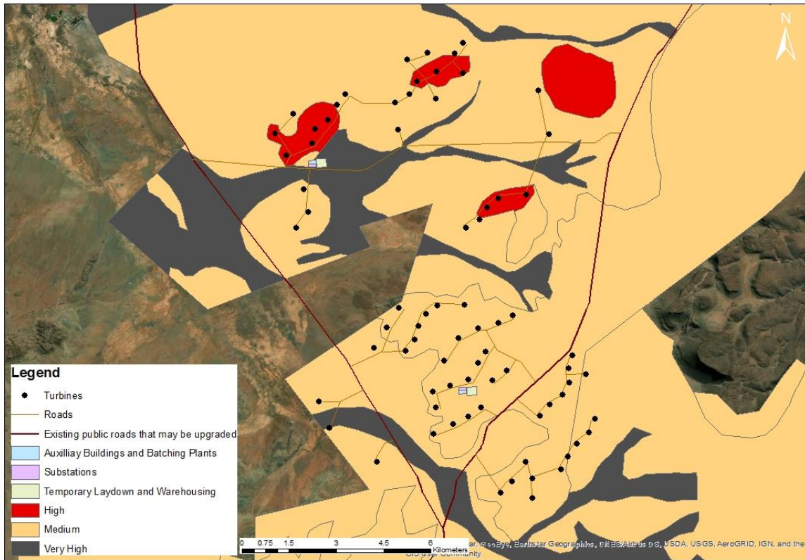
..... 51 Figure 5.1: Sensitivity map for faunal habitat within the site..... 51
