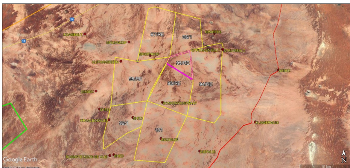
Figure 3.2: Red Sands SEFs site (pink) in relation to settlement pattern, adjacent properties (yellow), Aggenys-Gamoep public gravel road (red), existing Eskom lines (orange), and operational Kangnas WEF (green).
